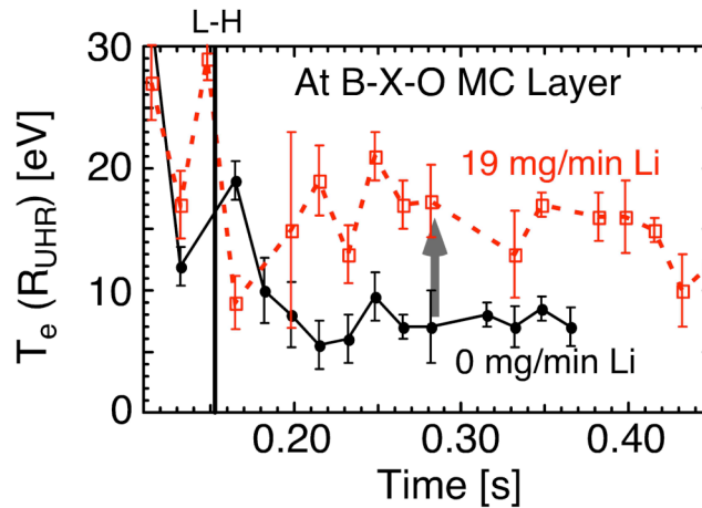
FIG. 7. The time evolution of T_e , measured by laser Thomson scattering, at the MC layer (where \omega = \omega_{UHR} ) is shown for a plasma without Li conditioning (solid line) and with Li conditioning (dashed line). The solid vertical line indicates the L-H transition while the vertical error bars represent the uncertainty in the Thomson scattering measurement.
