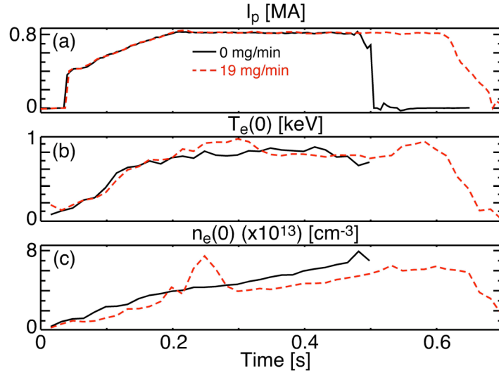
FIG. 5. The time evolution of (a) I_p , (b) T_e(0) , and (c) n_e(0) are shown for the target H-mode plasmas for the cases with 0 (solid line, no Li) and 19 mg/min (dashed line) of evaporated Li. The L-H transition occurs at 0.145 s.
