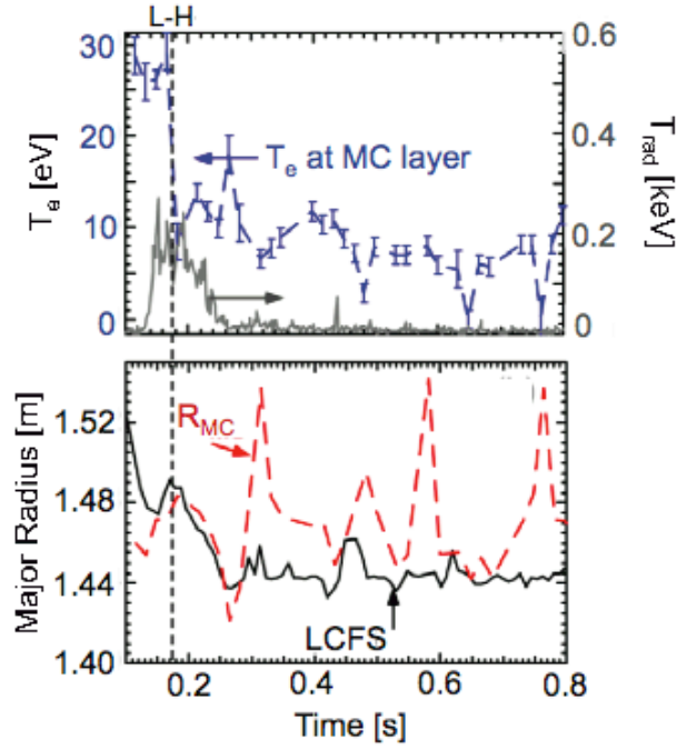
FIG. 2. (top) The time evolution of T_e at the MC layer (dashed line) and the measured radiation temperature, T_{rad} , (solid line) are shown. The vertical error bars represent the error in the Thomson scattering measurements. (bottom) The time evolution of the location of the last closed flux surface (solid line) and the position of the mode conversion layer, R_{MC} , (dashed line) are shown. The vertical dashed line indicates the L-H transition time.
