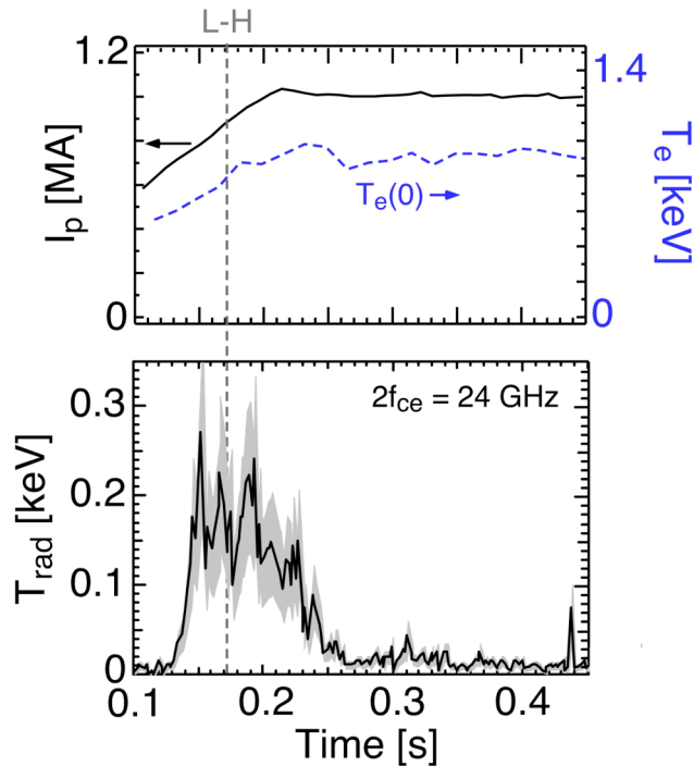
FIG. 1. (top) The I_p (solid line) and central T_e (dashed line) are shown as a function of time for an H-mode discharge. (bottom) The time evolution of second harmonic emission at 24 GHz, from near the plasma magnetic axis, is shown for an H-mode discharge. The shaded region represents the uncertainty in the measured T_{\text{rad}} .
