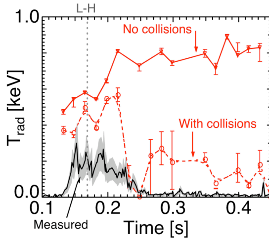
FIG. 3. EBE simulations of the low emission H-mode data, with (dashed line) and without (solid line) collisional damping effects. The error bars represent the uncertainty in the simulations due to errors in n_e and T_e from Thomson scattering as well as the magnetic equilibrium reconstruction.
