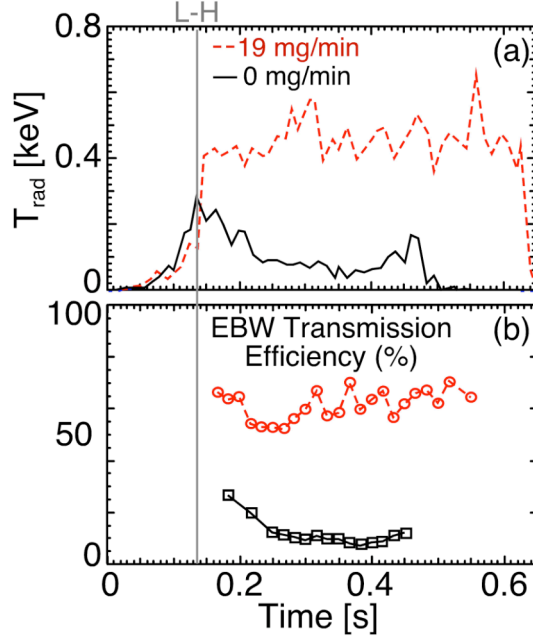
FIG. 8. (a) The measured T_{rad} and (b) B-X-O transmission efficiency are plotted for fundamental EBE (at 18 GHz) for Li evaporation rates of 0 mg/min (solid line) and 19 mg/min (dashed line).
