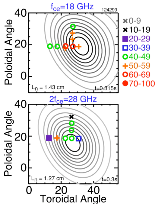
FIG. 10. Experimentally measured B-X-O transmission efficiency map (symbols) in a Li conditioned H-mode plasma for (a) f_{ce} = 18 GHz and (b) 2f_{ce} = 28 GHz. The contours represent the theoretical B-X-O transmission efficiency (equation 1), where the center represents 90% transmission. Subsequent contours represent a 10% decrease in transmission.
