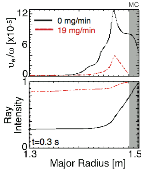
FIG. 9. The ratio of v_{ei}/\omega (top) and the intensity of the central ray (bottom) from the EBE simulation of a plasma without Li conditioning (solid line) and one with Li conditioning (dashed line) are shown as a function of major radius. The shaded region indicated the location of the MC layer.
