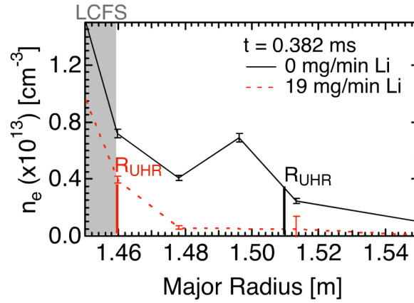
FIG. 6. The n_e profile from Thomson scattering is shown as a function of major radius in the plasma scrape off for two cases: no evaporated Li (solid line) and with 19 mg/min of evaporated Li (dashed line).
