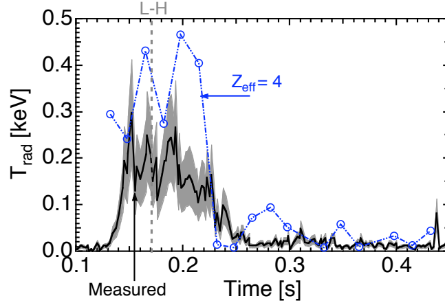
FIG. 4. EBE simulations of the low emission H-mode data with collisional effects, assuming Z_{\text{eff}} = 4 .
