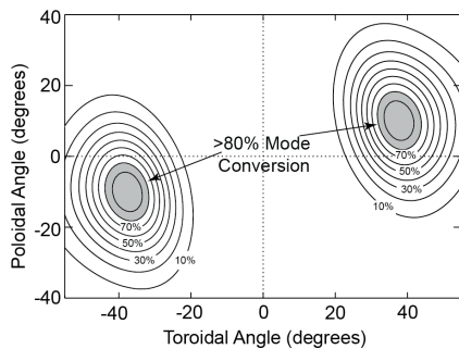
Figure 7.2.4: O-X-B mode conversion efficiency versus poloidal and toroidal angle for NSTX-U TRANSP run 142301V11 at 11.875 s. GENRAY-ADJ modeling was performed assuming a launched n_{||} = \pm 0.7 , corresponding to alignment of the mirror launcher with the indicated regions of maximum mode conversion.
