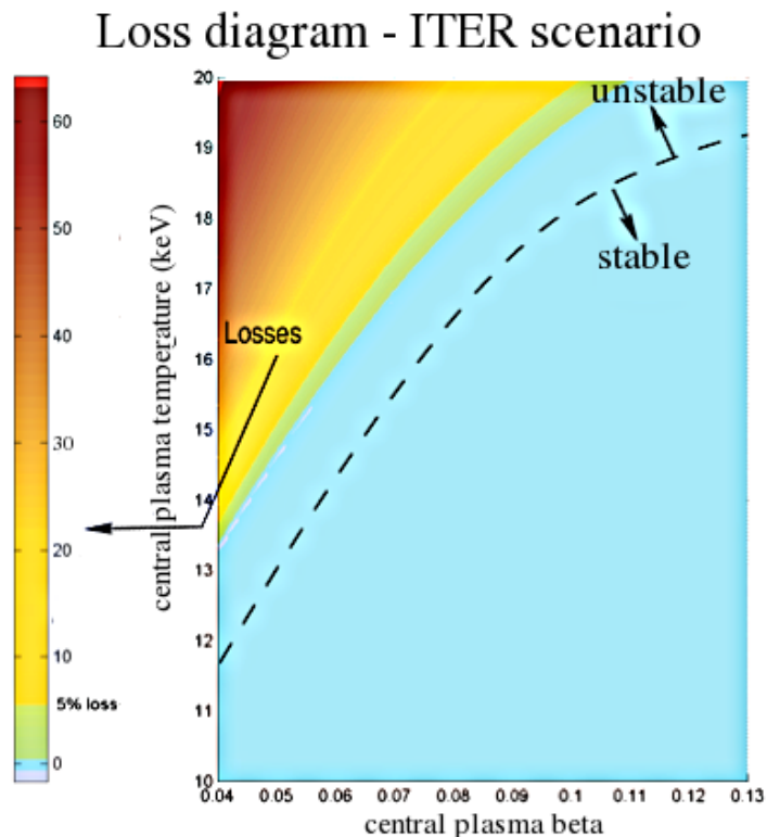
Figure 6.4.3: Example of quasi-linear model predictions of TAE stability for nominal ITER scenarios. On the abscissa is the central value of the plasma beta and on the ordinate is the central plasma temperature. TAE stability regions are indicated, along with the amount of losses expected in the presence of unstable modes.
