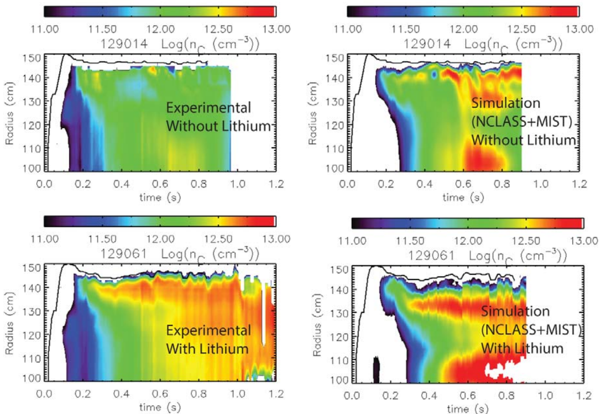
Fig. 3.3.16.. Evolution of the carbon density profile vs time and radius for the experimental measurements in a NSTX H-mode plasma (left panel; boronized discharge- TOP - lithiated discharge - BOTTOM), predictive MIST calculation (right panel; boronized discharge- TOP - lithiated discharge - BOTTOM).
