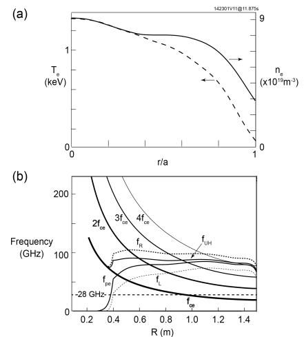
Figure 7.2.3: (a) Profiles of electron temperature (dashed line) and electron density (solid line) used for modeling EBW heating and current drive, and (b) electron cyclotron resonances and cutoffs for NSTX-U TRANSP run 142301V11 at 11.875 s.
