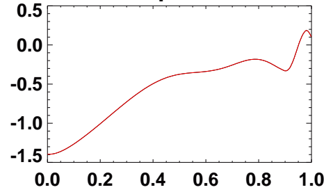
p and p' profiles
