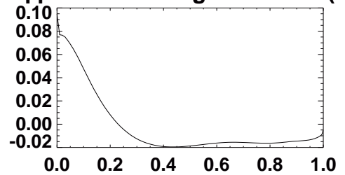
F profile convergence error (%)
