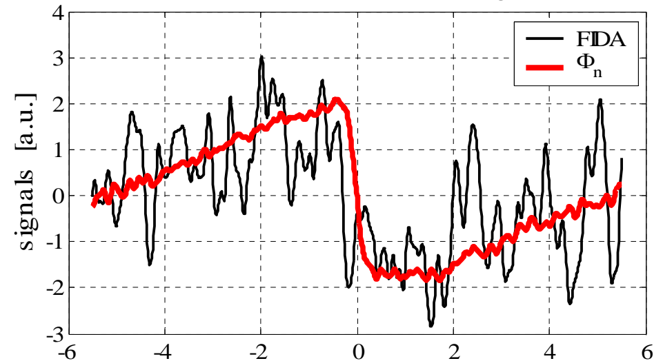
sh#124927 → 124939 conditional average of raw traces
