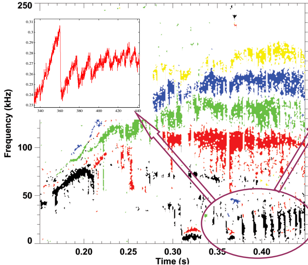
Shot 124938 \omega B(\omega) spectrum for toroidal mode number:
