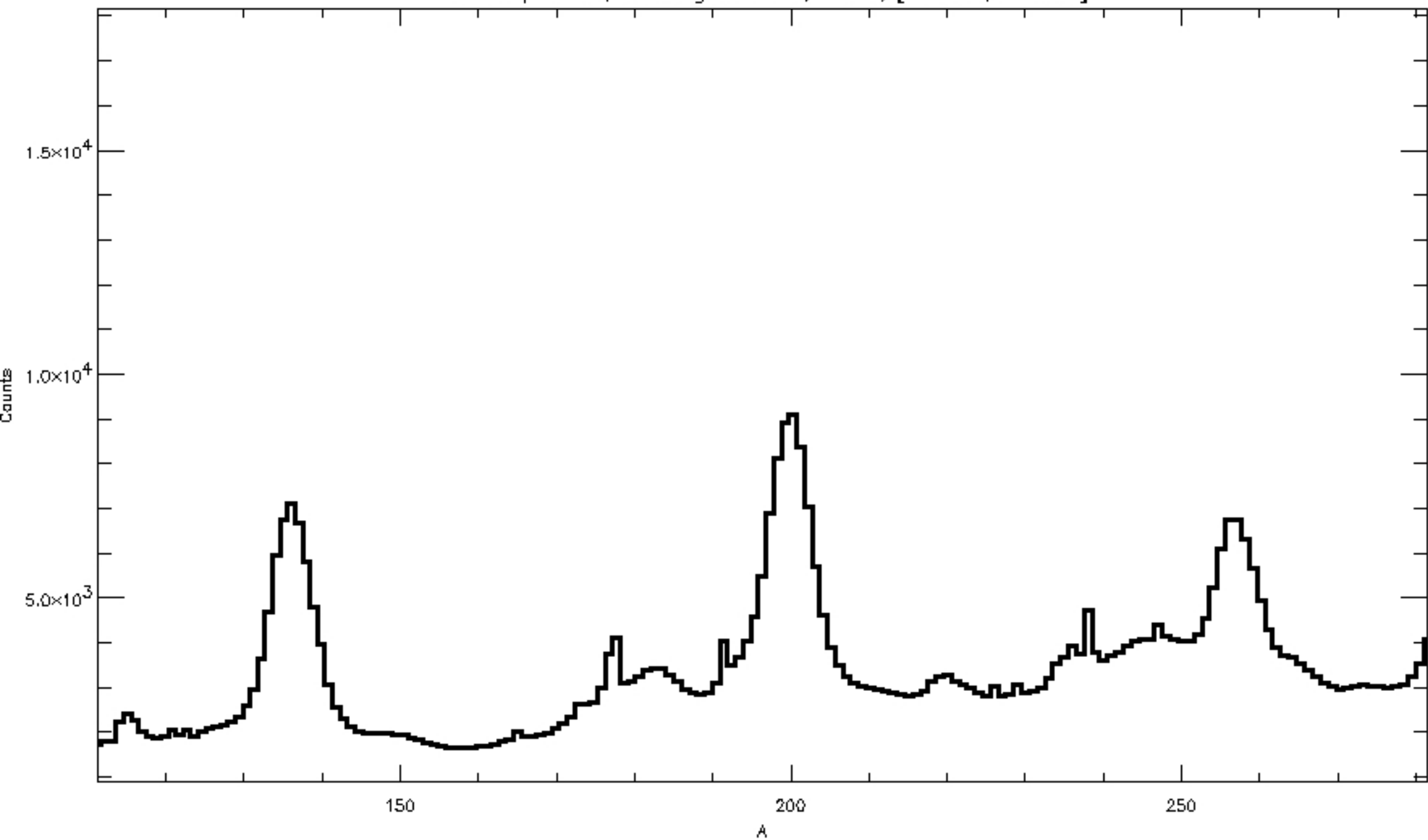
SPRED spectrum, discharge 124923, Bin: 7, [0.254 s, 0.266 s]
