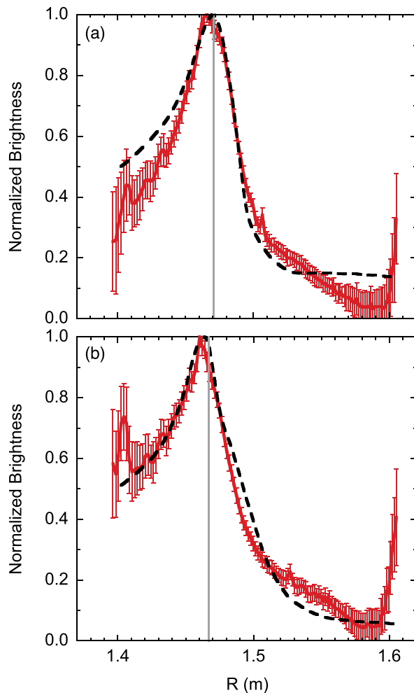
FIG. 3. Simulated (dashed) and observed (solid) radial ENDD profiles of line integrated Balmer- \beta brightness for shots (a) 139412 and (b) 142214, all normalized to maximum values of unity. The horizontal axis corresponds to the tangency radius of each pixel chord as obtained via Abel inversion. 12 The gray lines indicate the separatrix location at the Z coordinate of the ENDD view. The error bars on the experimental profile are associated with the calibration of the ENDD camera. Reprinted with permission from Stotler et al. , J. Nucl. Mater. 463 , 897 (2015). Copyright (2015) Elsevier.
