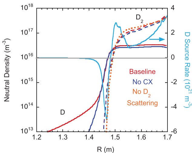
FIG. 11. Comparison of scaled neutral densities (left axis) in variants of the simulation of 142214 (red curves) without atom-ion charge exchange (blue curves) and without molecule-ion elastic scattering (orange dotted curve). The right axis depicts the volumetric source/sink rate of deuterium atoms in the baseline simulation across this radial slice.
