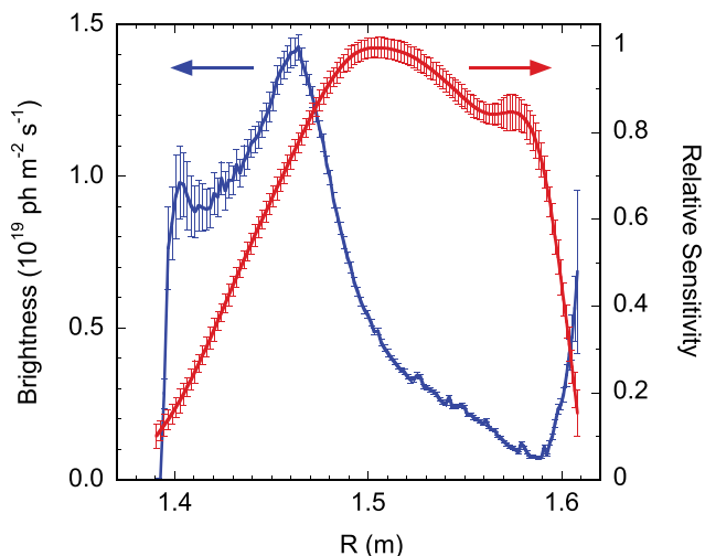
FIG. 7. Relative sensitivity of the ENDD imaging system is plotted on the right axis. The ENDD brightness profiles for shot 142214 are included for reference.
