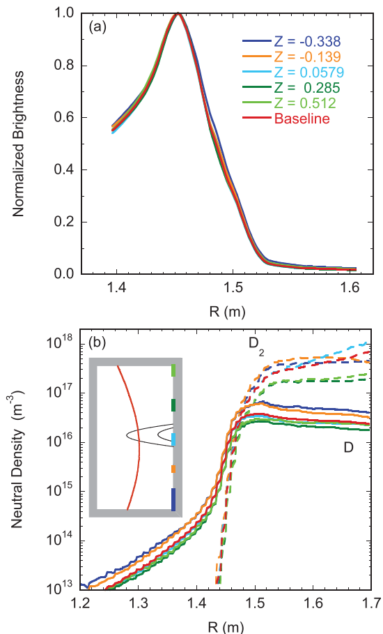
FIG. 9. Variation of (a) ENDD and (b) density profiles with source location on outer wall.
