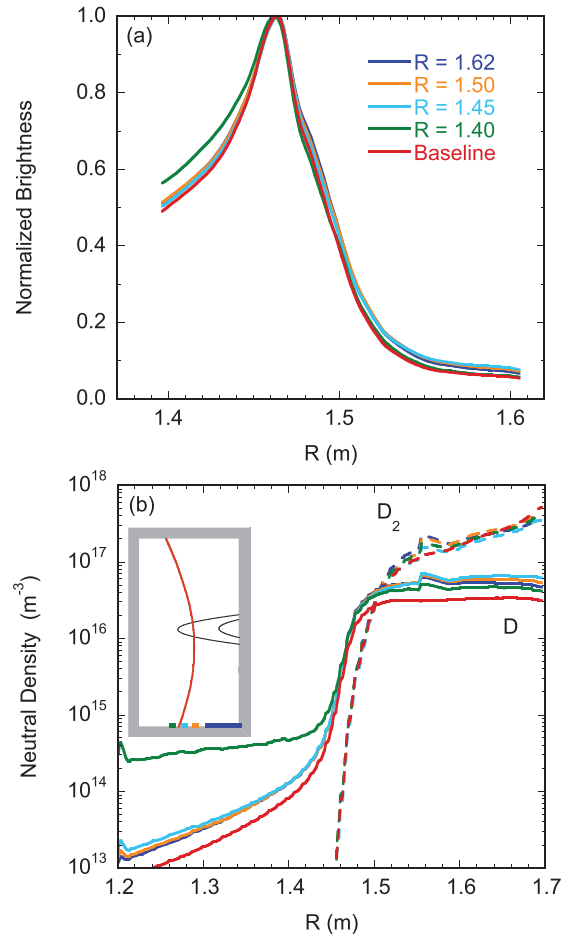
FIG. 10. Variation of (a) ENDD and (b) density profiles with source location on lower wall.
