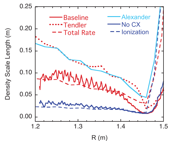
FIG. 12. Scale lengths for the deuterium atom density, \lambda \equiv (dn_{\text{D}}/dR)^{-1} , for the baseline simulation of shot 142214 (solid red line) and for the variant without atom-ion charge exchange (solid blue line). The scale length derived in Ref. 46 evaluated with the neutral thermal velocity equal to the ion thermal velocity is labeled “Tendler” (red dotted line). “Total Rate” (red dashed line) is a simpler variant, Eq. (6). The curve labeled “Alexander” (solid cyan) is computed using Eq. (7). The dashed blue line is the penetration length computed from the ionization rate at an energy of 3 eV.
