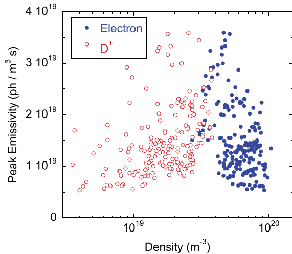
FIG. 2. Relationships between the peak of the ENDD emissivity profiles for all time slices and the maximum electron density (from Thomson scattering profiles) and edge deuterium ion density (from CHERS).
