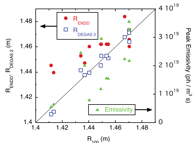
FIG. 4. Simulated ( R_{\text{DEGA2}} ; squares) and observed ( R_{\text{ENDD}} ; circles) locations of the peaks in the ENDD profiles as a function of the midplane major radius at which T_e = 100 eV, R_{100} . The peak emissivity (triangles, right axis) tends to increase with R_{100} .
