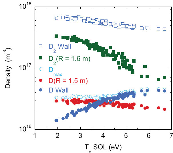
FIG. 8. Relationship between neutral densities and the assumed SOL electron temperature in the Monte Carlo sampled simulations described in Sec. VB 1. Molecular densities at the wall ( R = 1.7 m) and at R = 1.6 m are shown. The maximum atomic density over the profile, D_{\max} is depicted, as are the values at R = 1.5 and 1.7 m.
