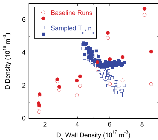
FIG. 6. Range of atomic (vertical axis) and molecular (horizontal axis) densities for all baseline simulations (circles). Both the atomic densities at the wall (closed symbols) and profile maxima (open symbols) are depicted. The squares are the atomic and molecular densities for the 100 simulations with the Monte Carlo sampled n_e and T_e profiles of shot 142214 at 0.4 s, described in Sec. VB 1.
