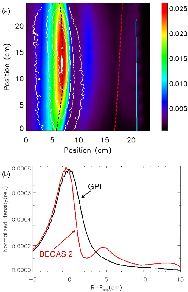
FIG. 8. Comparison between the time-averaged D\alpha light emission measured in NSTX and the calculated emission in the DEGAS 2 simulation of the NSTX edge plasma and the GPI view. [Reproduced with permission from Fig. 4 of Cao et al. , Fusion Sci. Technol. 64 , 29 (2013). Copyright 2013 American Nuclear Society.] The color contours are the DEGAS 2 results and the equally spaced white contours are the GPI results, the leftmost dashed line is the separatrix, the rightmost dashed line is the limiter shadow, and the nearly vertical line is the gas manifold. The 1-D profiles are obtained by normalizing the 2-D data to the sum over all pixels and then averaging over vertical pixels. The horizontal coordinate is mapped to the outer midplane separatrix.
