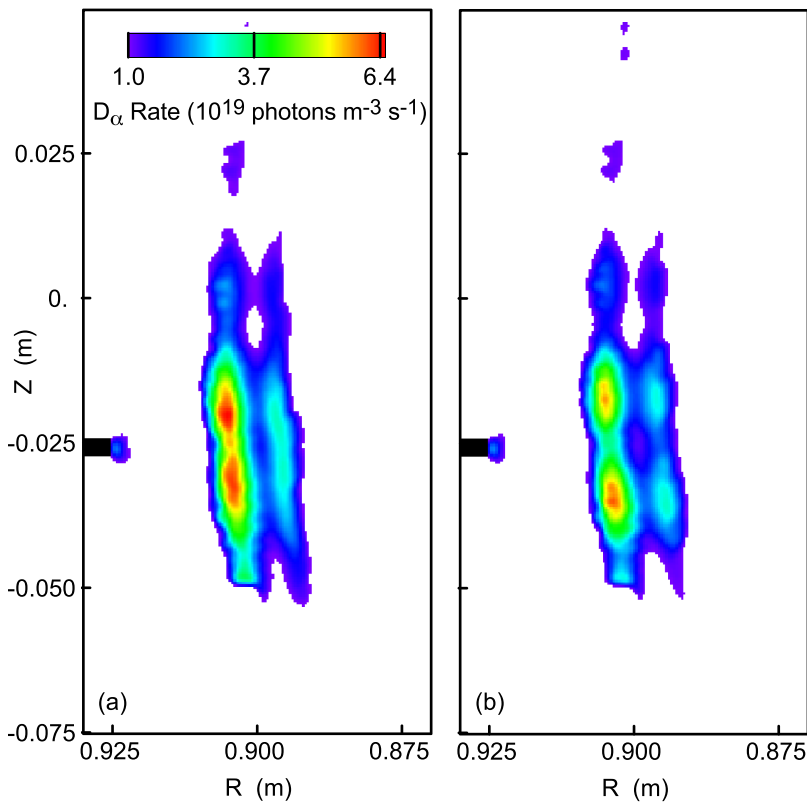
FIG. 10. DEGAS 2 simulations of the D_{\alpha} light emission patterns in GPI in Alcator C-Mod assuming a strong poloidal and radial modulation of the electron density. [Reproduced with permission from J. Nucl. Mater. 313-316 , 1066 (2003). Copyright 2003 AIP Publishing LLC.] The gas nozzle is shown as a black rectangle in the left. In (a) the shadowing effect of the fluctuations on the neutral density is incorporated, and in (b) the shadowing effect has been eliminated using post-processing. The result is that the spatial structure of the emission profile in (a) is smeared out relative to the idealized result shown in (b) and relative to that of the perturbed density.
