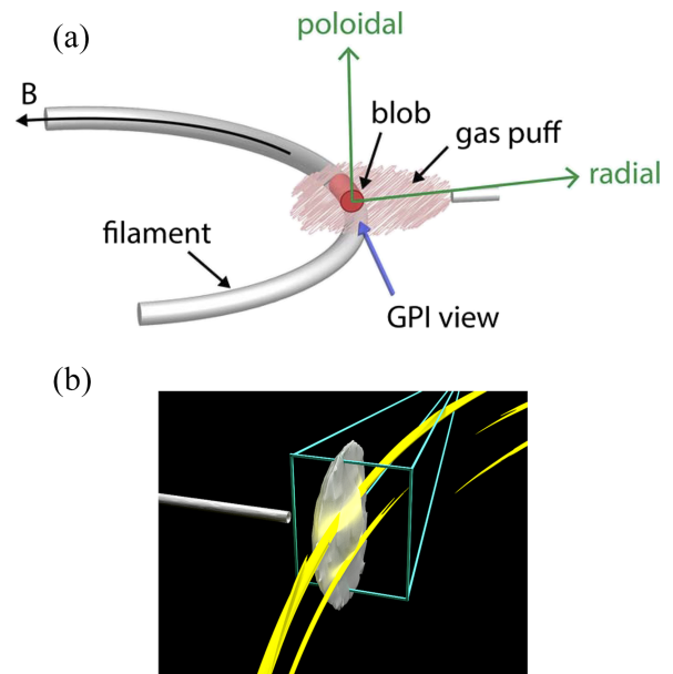
FIG. 1. Gas puff imaging (GPI) geometry in a tokamak. The simplified picture in (a) shows a single 3-D plasma edge filament aligned along the magnetic field direction B , along with a schematic illustration of a gas puff cloud. [Reproduced with permission from Fig. 1 of Cao et al. , Fusion Sci. Technol. 64 , 29 (2013). Copyright 2013 American Nuclear Society.] When viewed along the local B field direction in the cloud, the 2-D structure of the filament perpendicular to B should be fairly clearly visible (i.e., the “blob”). The more realistic image in (b) was constructed using plasma turbulence simulation outputs of XGC-1 and gas cloud outputs from DEGAS 2 [visualization provided by D. Pugmire, private communication (2016)]. 169 The yellow filaments are edge density structures near the separatrix in the XGC-1 output, which are aligned along the magnetic field. The gray is the GPI gas cloud shape from DEGAS 2, and the yellow glow is where the filaments intersect the computed gas cloud. The blue box is the simulated GPI camera view, and the tube at the left is the GPI gas puffer.
