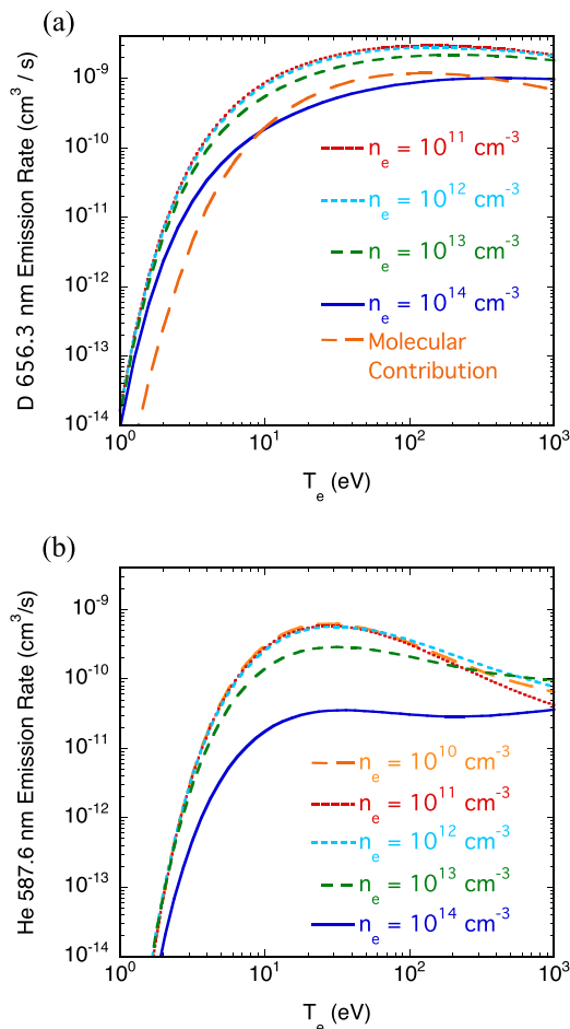
FIG. 6. (a) Deuterium Balmer- \alpha (656.3 nm) and (b) HeI 587.6 nm photon emission rate per electron per neutral atom, i.e., f(n_e, T_e)/n_e in Eq. (3) obtained from the collisional radiative model described in the text. The photon emission rate per electron per deuterium molecule is included in (a) for comparison; these contributions are described in Sec. V C.
