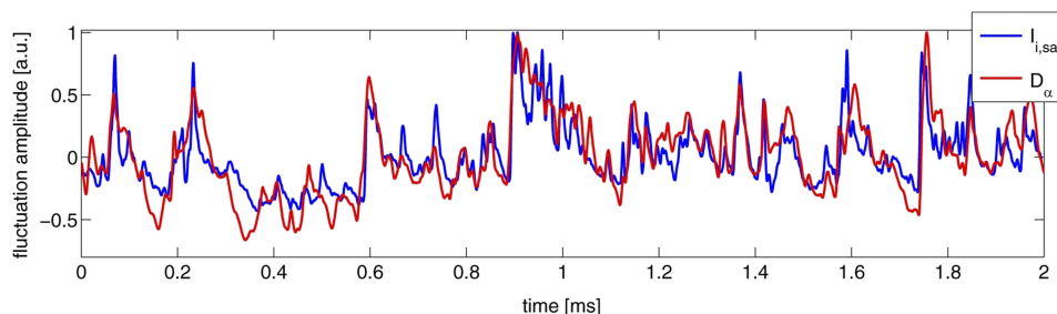
FIG. 9. A \sim 2 ms long time series of ion saturation current fluctuations measured with a reciprocating probe in Alcator C-Mod (blue), overlaid with a GPI signal from a single view within the 2-D array of APD views at outer midplane. [Reproduced with permission from Fig. 5 of Grulke et al. , Nucl. Fusion 54 , 043012 (2014). Copyright 2014 IOP Publishing.] These two diagnostics sample the same flux-tube, but displaced by \sim 2.8 m along B. It is clearly seen that fluctuation events are observed by both diagnostics, and large-amplitude events especially can be directly identified in both traces. The cross-correlation amplitudes between the GPI emission and I_{\text{sat}} of over 75% are found in some cases. A small -1.5 \pm 0.5 \mu\text{s} time delay maximizes the cross-correlation between the two time-series.
