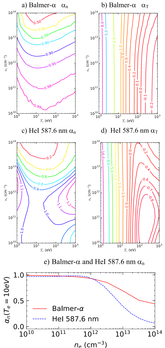
FIG. 7. (a) Density and (b) temperature exponents \alpha_n and \alpha_T as defined in Eq. (5) for the deuterium Balmer- \alpha (656.3 nm) data shown in Fig. 6(a). (c) and (d) are the analogous quantities for HeI (587.6 nm). (e) Density exponent variation with respect to n_e at T_e = 10 eV.
