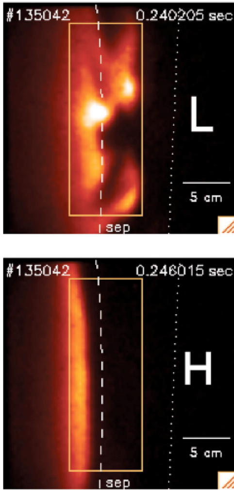
FIG. 2. GPI images from the NSTX tokamak made near the outer midplane over a 24\text{ cm} \times 24\text{ cm} region using a \text{D}_2 gas with a Balmer- \alpha filter and a 2.1\ \mu\text{s} camera exposure time. [Reproduced with permission from Phys. Plasmas 17 , 102502 (2010). Copyright 2010 AIP Publishing LLC.] At the top is a typical L-mode plasma, and at the bottom is a quiescent H-mode plasma later in the same shot. In both cases the raw camera data are displayed using the same false linear color scale (white as maximum and black as zero), with the poloidal direction vertical, the radial direction horizontal (outward to the right), and the magnetic separatrix from the EFIT reconstruction is shown by the dashed line. The data are analyzed only within the orange boxes since \text{D}\alpha emission is too small in the low electron temperatures near the wall (right of the box), and also too low farther inside the plasma where the ionization occurs at high temperatures (left of the box).
