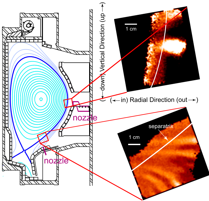
FIG. 3. GPI images from the Alcator C-Mod tokamak made at two different 6\text{ cm} \times 6\text{ cm} regions using \text{D}_2 gas with the Balmer- \alpha line filter. The imaged regions are shown schematically along with the plasma equilibrium at the time when the image from outboard of the lower X-point was taken. 45 The other imaged region is at the low-field-side midplane. The four-hole nozzle at the LFS midplane and the single-hole nozzle in the outer divertor target, below the lower imaged region, are also shown. These images are normalized with respect to the time-averaged images of each region to show the structure of the relative fluctuation levels , where white is 1.5 and black is 0.5, and the low signal region well inside the separatrix is forced black. The maximum fluctuation levels are large ( \pm 50\% ) in both locations, and the structures in the X-point region are significantly tilted with respect to the local separatrix. Both discharges are in H-mode.
