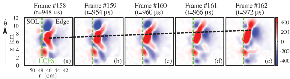
FIG. 4. A time sequence of GPI images from the TEXTOR tokamak made with camera exposure times of 6\ \mu\text{s} each over a 12\text{ cm} \times 12\text{ cm} region at the outer midplane using \text{D}_2 gas with a \text{D}\alpha filter. [Reproduced with permission from Rev. Sci. Instrum. 84 , 053510 (2013). Copyright 2013 AIP Publishing LLC.] These images have their time averages image subtracted to show more clearly the positive (red) and negative (blue) excursions from the mean signal. The poloidal motion of one positive structure is shown by the black dashed line, and the last closed flux surface is shown by the green dashed line, with the radially outward direction toward the left. These data are from an Ohmic discharge.
