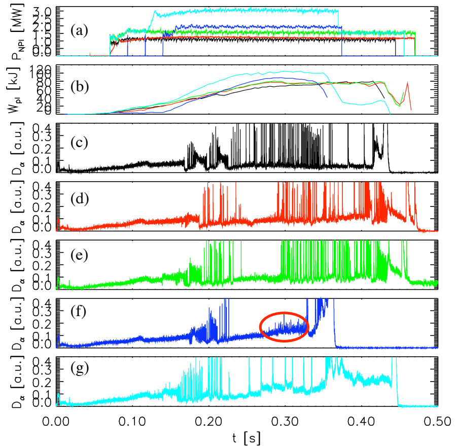
Fig. 4. Characteristics of MAST discharges with an NBI power scan. The NBI power is shown in panel (a), and plasma stored energy in panel (b), and the divertor D_\alpha characteristics of each discharges in the NBI scans in panels (c)-(g).
