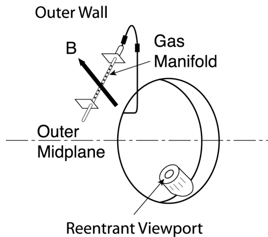
Fig. 7a. GPI setup on NSTX, showing camera view of gas manifold along B.
