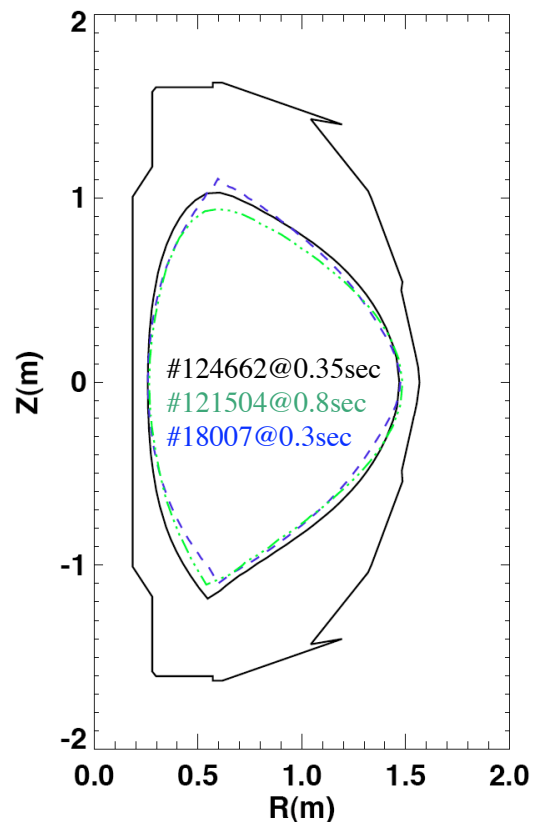
Fig. 1. Common shape developed for experiment. Color code: NSTX (black), MAST (blue: dashed), and C-Mod (green: dash-dot). The NSTX and C-Mod plots are scaled by 0.96 and 2.8 respectively, and the C-Mod boundary is shifted inward by 0.19 m.
