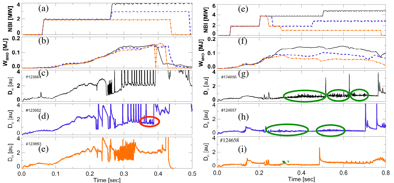
Fig. 6. Characteristics of NSTX discharges in power scan. The left panels (a)-(e) were taken with \delta_r^{\text{sep}} = -0.6\text{cm} , whereas the right panels (e)-(i) were with \delta_r^{\text{sep}} = -1.5\text{cm} and a lower X-point height. The red oval highlights small ELM in panel (d) and the green ovals Type V ELMs in panels g,h.
