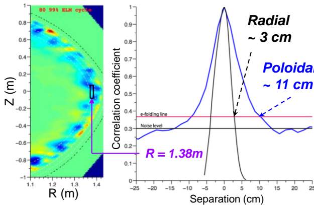
FIG. 7. Edge electrostatic potential fluctuations computed from XGC1 yield radial and poloidal correlation lengths in the range of measured values from reflectometry and BES diagnostics.
