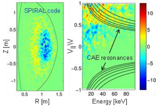
FIG. 15. Fast ion redistribution by saturated kink mode activity.
