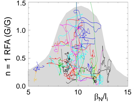
FIG. 9. n=1 resonant field amplification during high \beta discharges using active MHD spectroscopy, indicating improved stability at high \beta_N/l_i .
