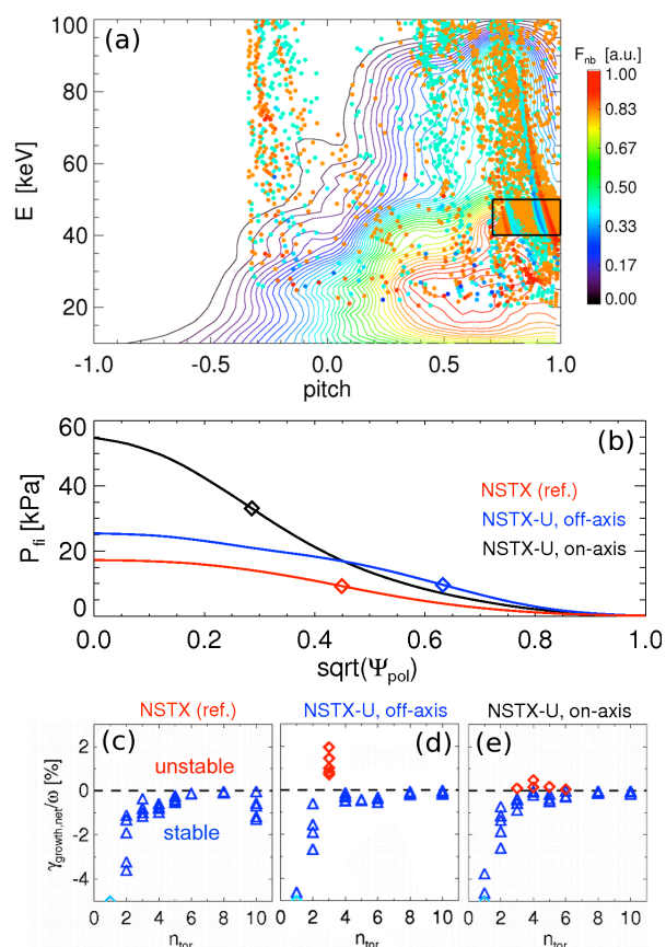
Fig. 2: (a) Fast ion distribution vs energy and pitch (ratio of parallel to total velocity). Red (blue) dots represent resonant particles which gain (lose) energy, as calculated by the ORBIT code. The rectangle delimits a region with enhanced resolution, showing the large number of possible resonances. (b) Fast ion pressure for a reference NSTX scenario and for NSTX-U projections with different NBI geometries. (c-e) NOVA-K stability results for the 5 least stable TAEs with toroidal mode number n=1\text{-}10 .
