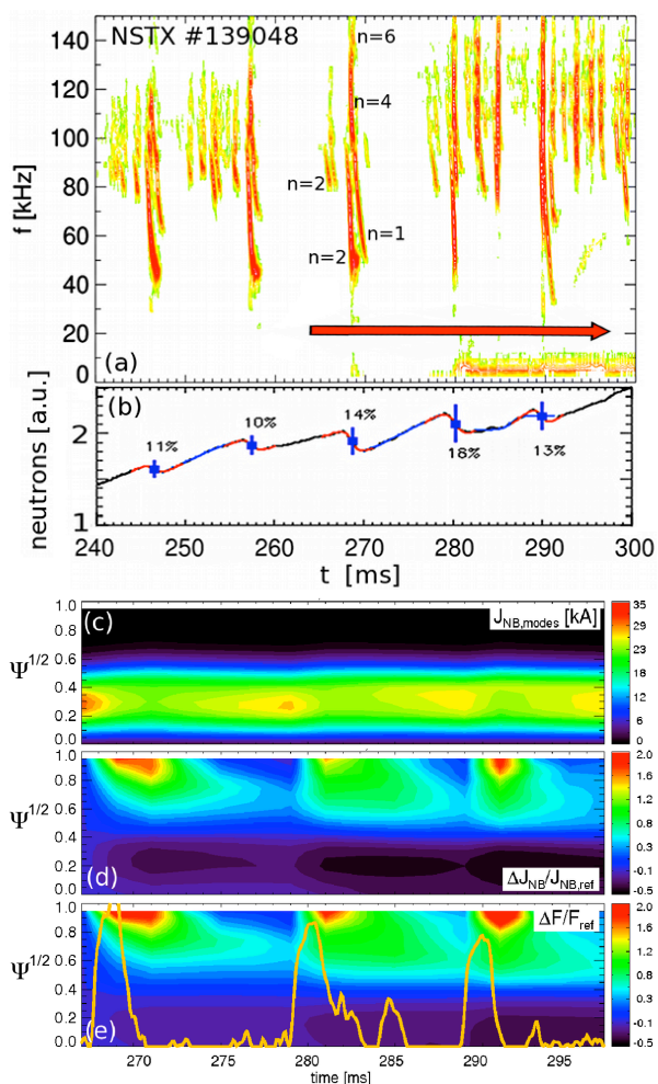
Fig. 1: (a) Spectrum of TAE and kink-like activity for NSTX discharge no. 139048. Red arrow shows the time of interest. (b) Measured neutron rate showing significant drops caused by TAEs. (c) Simulated evolution of NB-driven current. (d-e) Changes of NB-driven current and fast ion density relative to the case with no instabilities. Solid line in (e) shows the total TAE mode amplitude.
