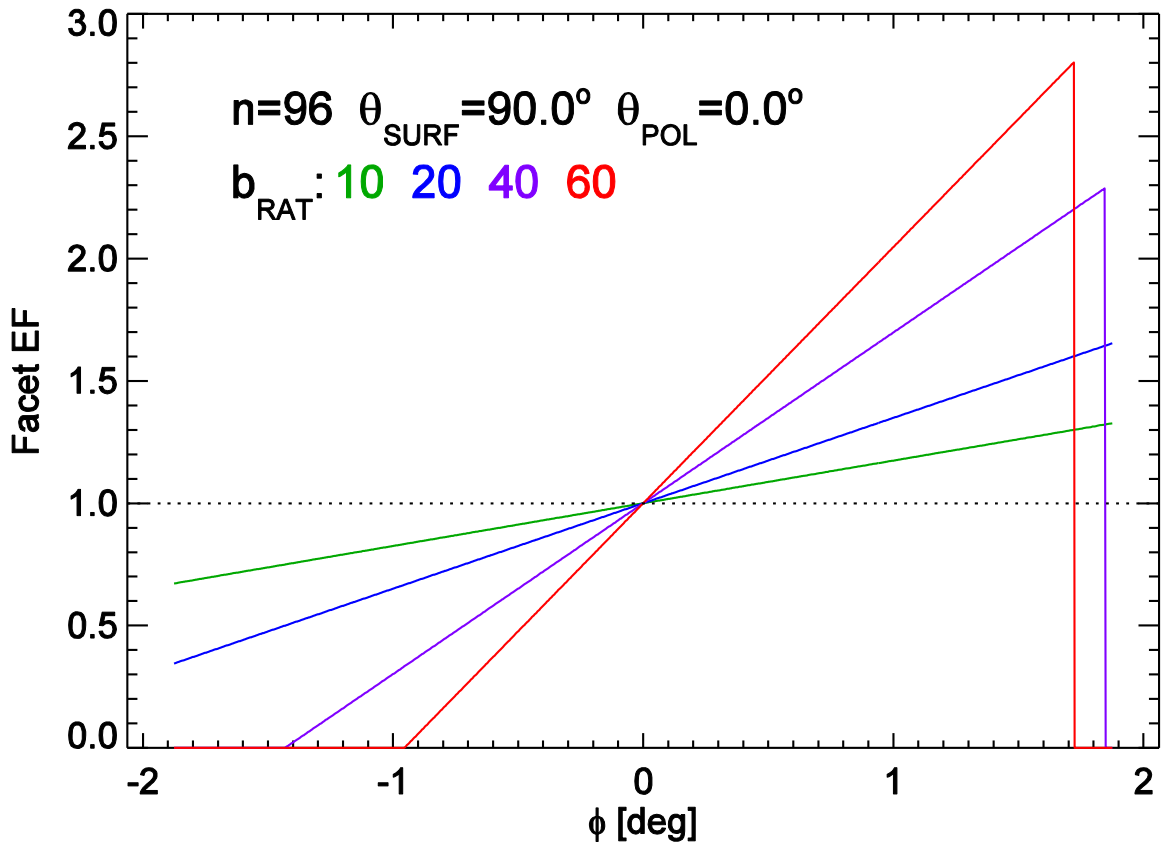
Figure 8: Calculation of heat flux enhancement factor, EF , for vertical plate, showing the shadowed regions for large values of b_{\text{rat}} .
