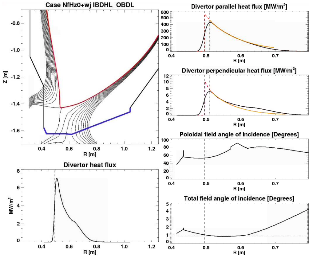
Fig. 5.1.4: Geometry and profiles from high flux expansion case 2.10.
