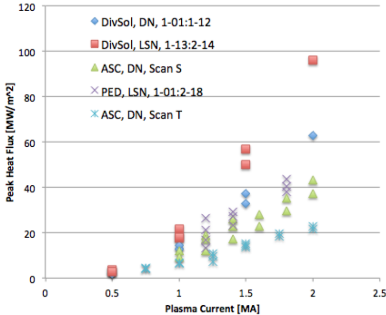
Fig. 4.3.1: Peak heat flux on the lower target as a function of plasma current, for the scans described in this section.
