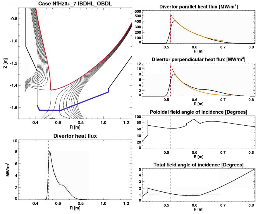
Fig. 5.1.3: Geometry and profiles from high flux expansion case 1.8.
