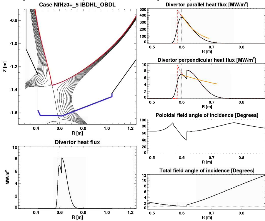
Fig. 5.2.2: Geometry and profiles from high flux expansion case 1.6.
