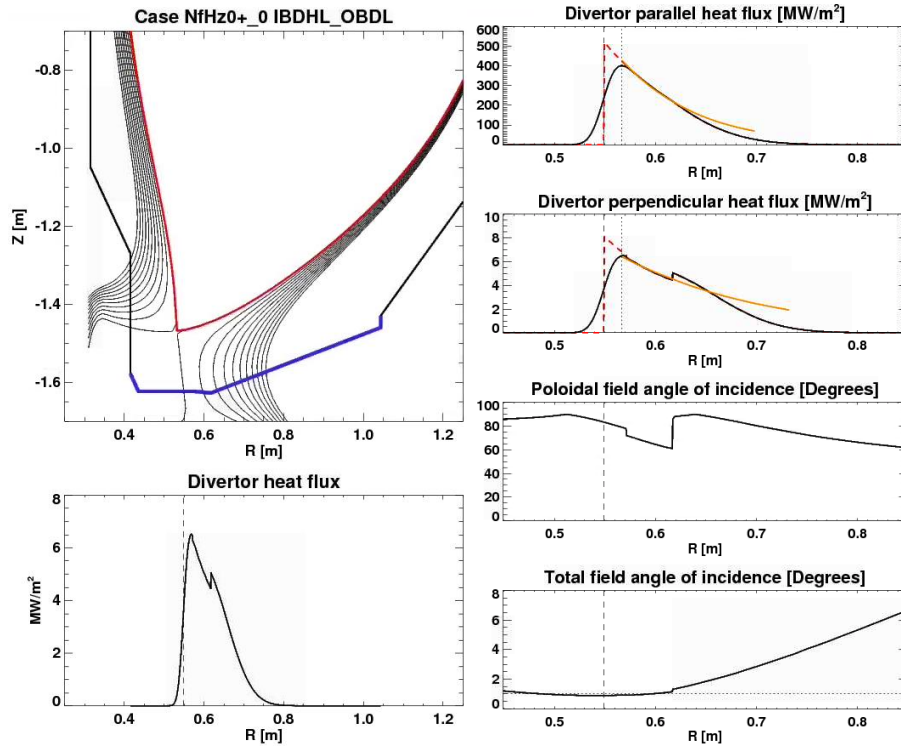
Fig. 5.1.1: Geometry and profiles from high flux expansion case 1.1.
