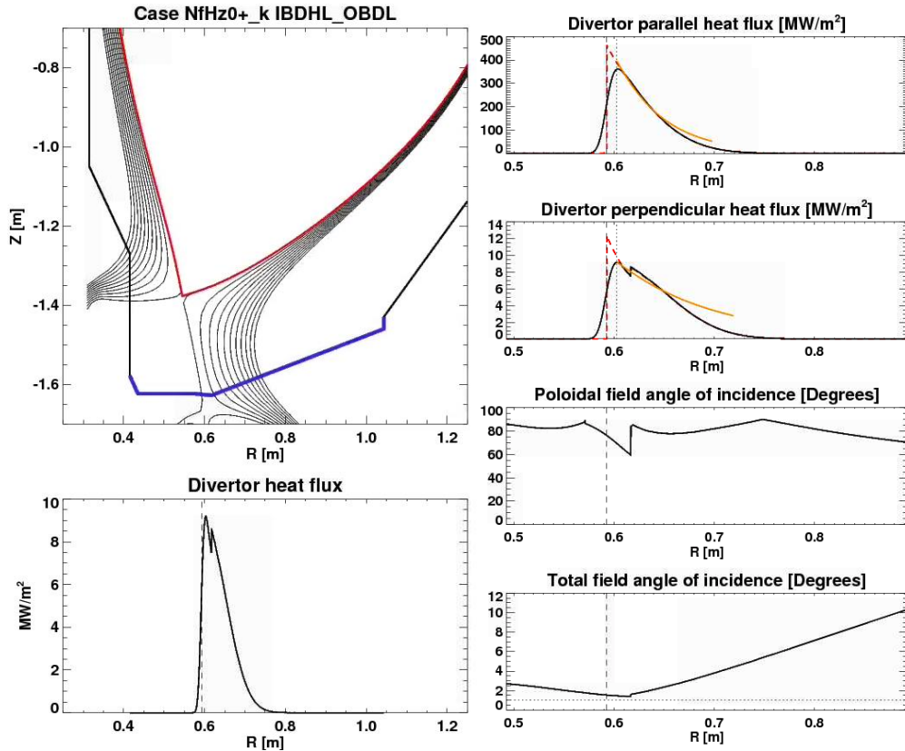
Fig. 5.2.1: Geometry and profiles from high flux expansion case 1.21.
