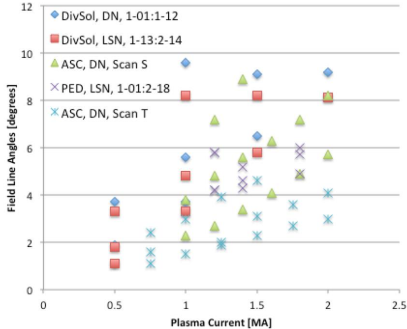
Fig. 4.3.2: Field line angle at the strikepoint as a function of plasma current, for the scans described in this section.
