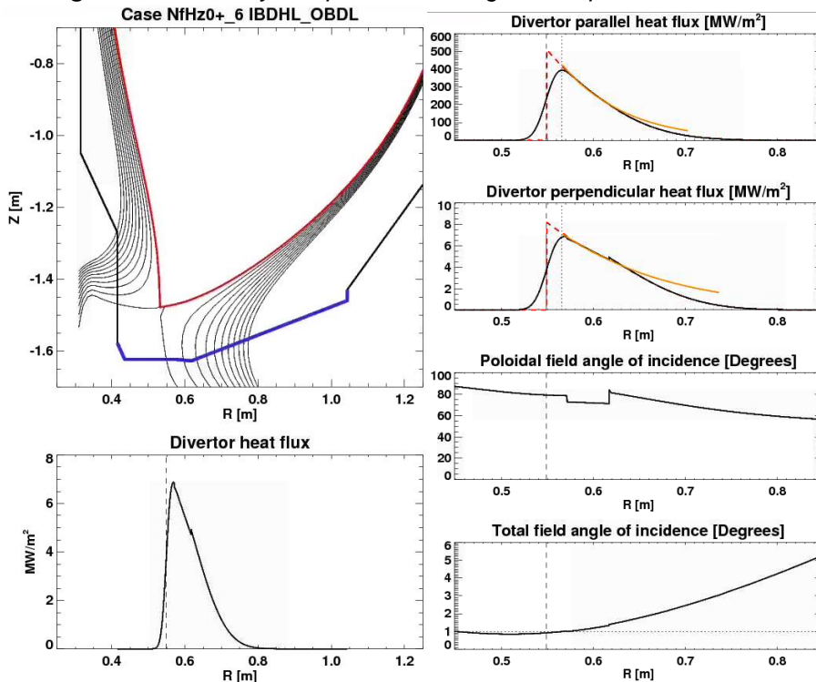
Fig. 5.1.2: Geometry and profiles from high flux expansion case 1.7.
