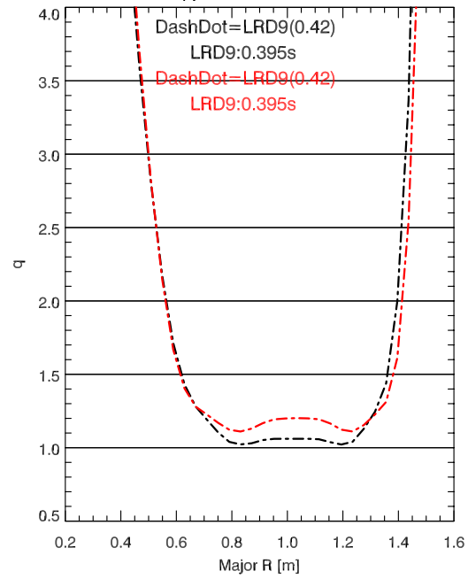
q profiles, t=0.395s
