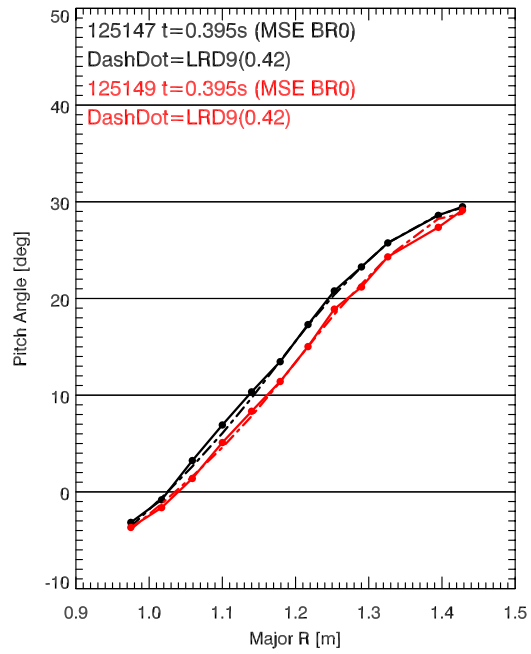
MSE E_r ( v_\phi only) Corrected Pitch Angle Profiles user_time=0.395s
