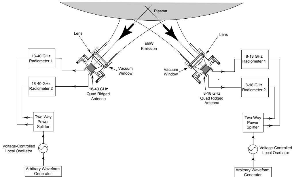
Figure 3. Machine layout of the upgraded remotely-steered EBW emission diagnostic. Each antenna is coupled to a dual channel, absolutely calibrated radiometer system. The 8-18 GHz radiometer will measure O-mode EBW emission in the fundamental frequency range while the 18-40 GHz radiometer will measure emission in the second harmonic frequency range.
