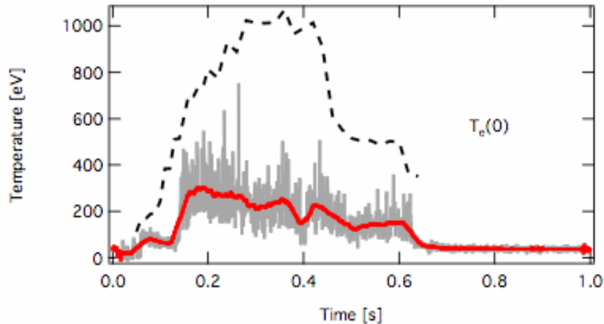
Figure 1. T_{\text{rad}} is plotted versus time for NSTX shot 117970. The grey trace is the radiation temperature obtained from the absolutely calibrated radiometer for 25 GHz emission. The red trace is the smoothed T_{\text{rad}} data. The black dashed line is the Thomson scattering electron temperature on axis.
