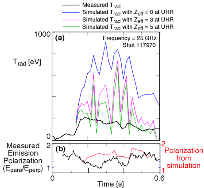
Figure 2. Measured T_{\text{rad}} and emission polarization for shot 117970 for 25 GHz. (a) T_{\text{rad}} vs. time is plotted. The black trace is the time-averaged measured emission. Also plotted is the simulated T_{\text{rad}} for shot 117970, the blue trace ( Z_{\text{eff}}=0 ) neglects the effects of collisions, the pink ( Z_{\text{eff}}=3 ) and green ( Z_{\text{eff}}=5 ) include collisional effects. (b) The black trace shows the measured emission polarization while the red trace shows the simulated emission polarization.
