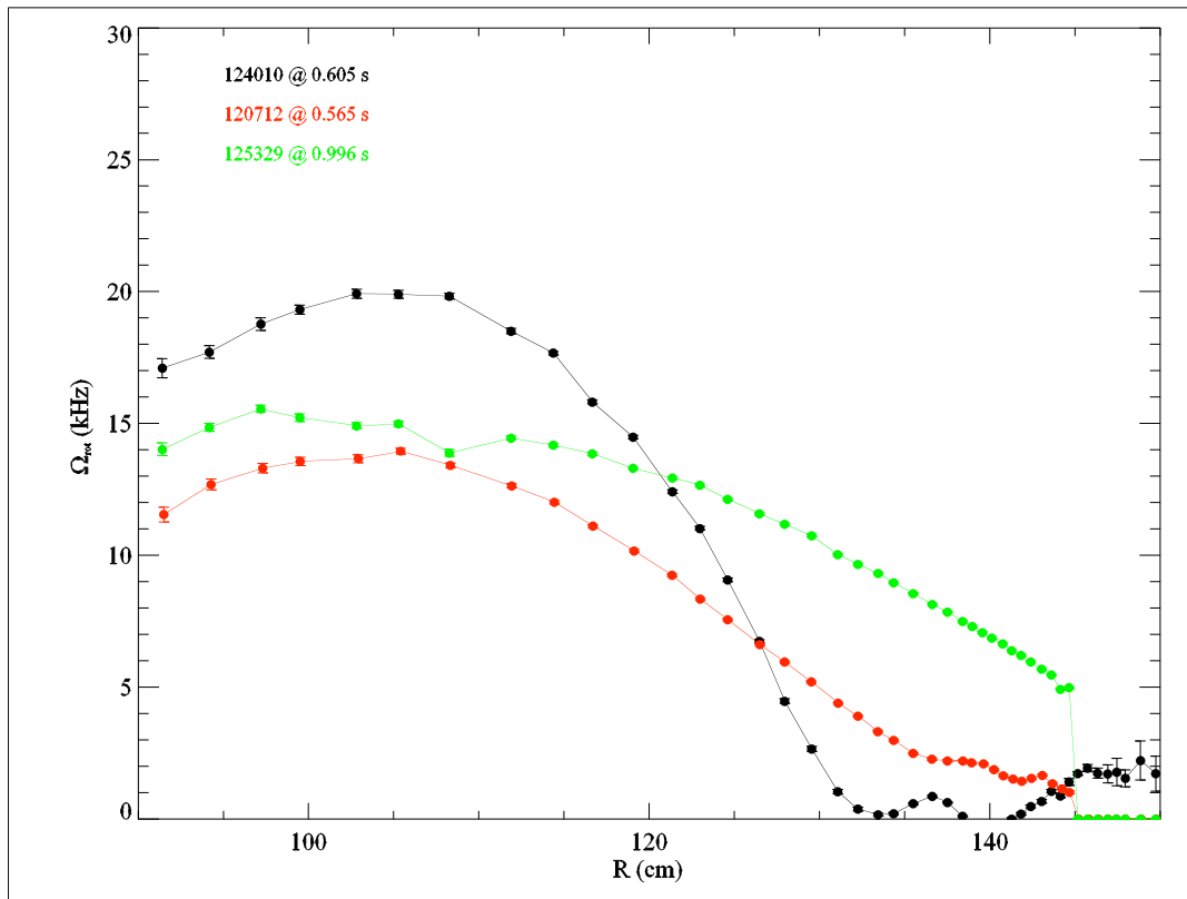
Figure 2: Comparison of rotation profile for three different shots.
