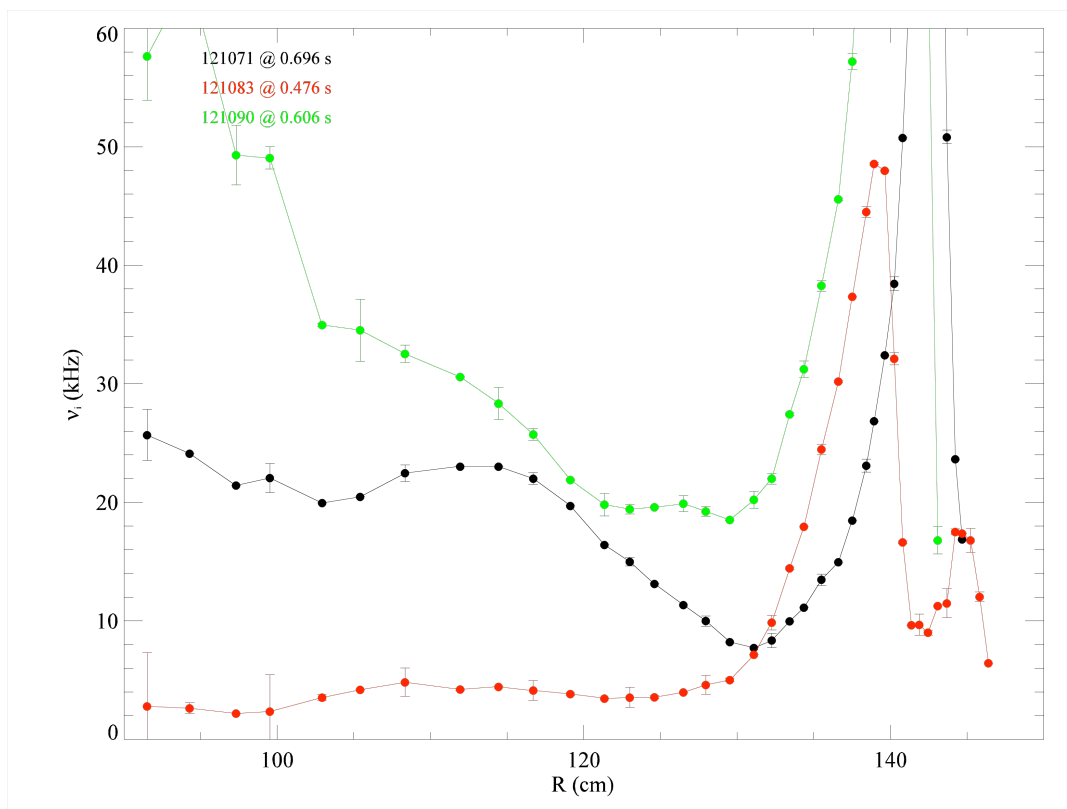
Figure 3: Comparison of ion collisionality for three different shots just before RWM instability.
