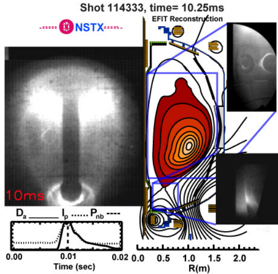
Fig. 1. Data from three cameras combined with an EFIT reconstruction [10] and plots of other plasma conditions vs. time. As time progresses in the composed animation, the vertical dashed line on the plasma-conditions vs. time plot moves to the right, and individual frames from each camera and the flux contours from EFIT, are displayed at the appropriate time.
