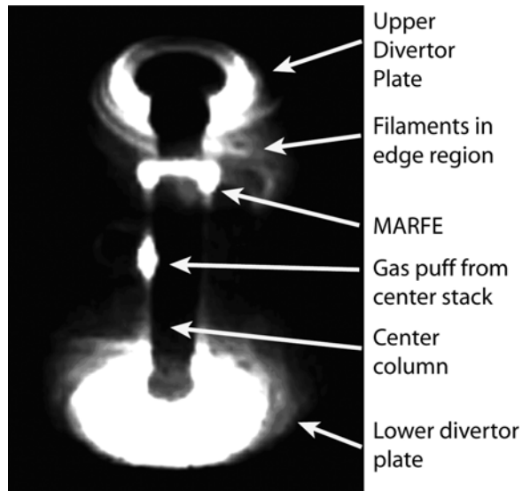
Fig. 2. 9 \mu sec exposure from a Phantom 7 Camera showing a MARFE on the center stack and fast filamentation on the edge (128x128 pixels, contrast enhanced).
