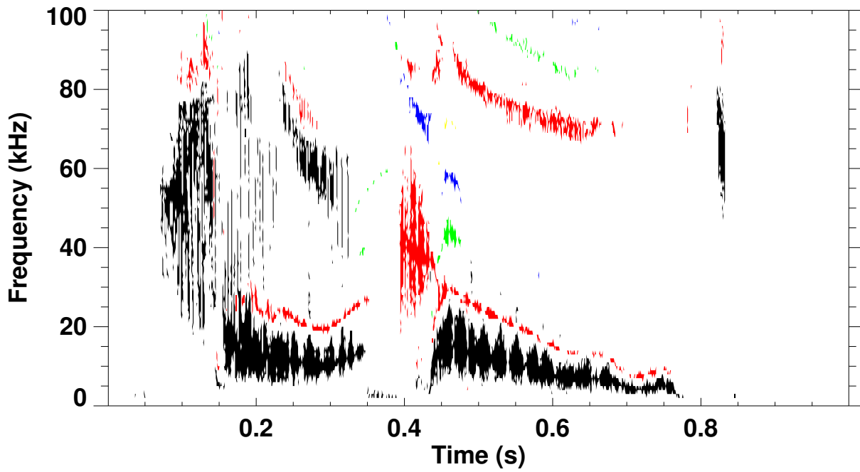
Shot 115789 \omega B(\omega) spectrum for toroidal mode number: 1 2 3 4 5
