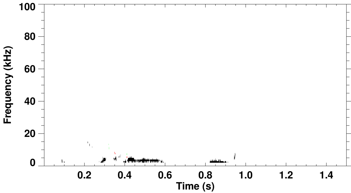
Shot 117597 \omega_B(\omega) spectrum for toroidal mode number: 1 2 3 4 5
