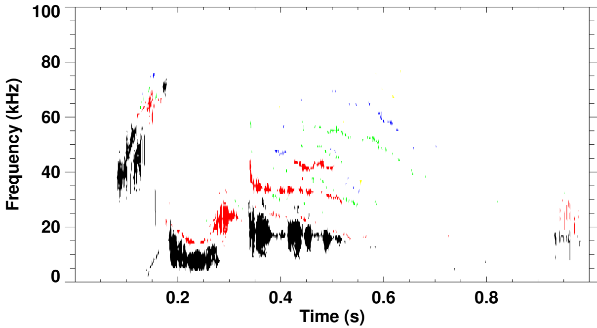
Shot 117707 \omega B(\omega) spectrum for toroidal mode number: 1 2 3 4 5
