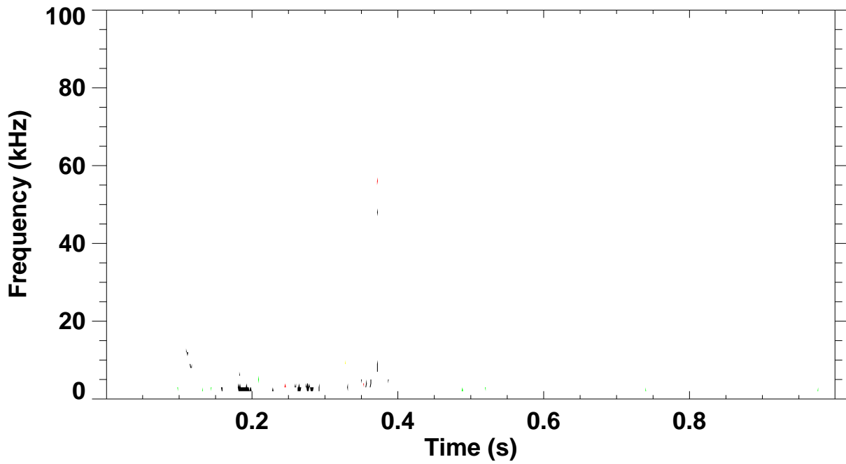
Shot 126591 \omega B(\omega) spectrum for toroidal mode number: 1 2 3 4 5
