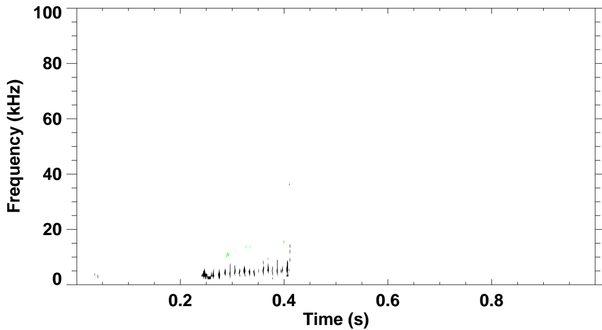
Shot 127080 \omega B(\omega) spectrum for toroidal mode number: 1 2 3 4 5
