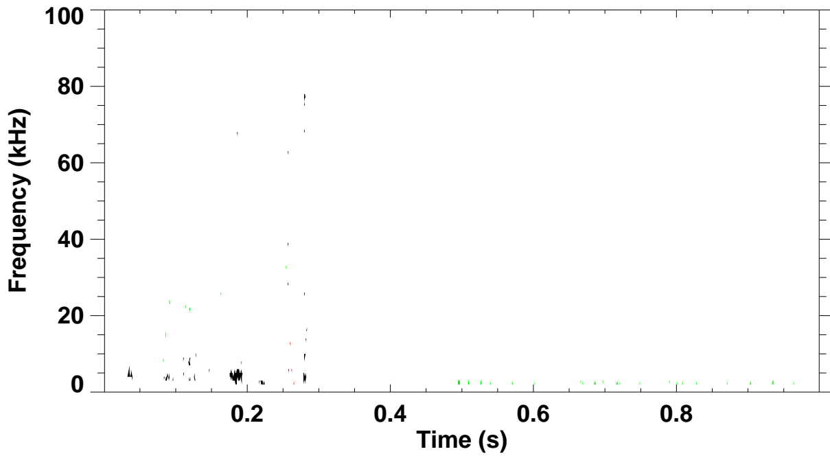
Shot 127108 \omega B(\omega) spectrum for toroidal mode number: 1 2 3 4 5
