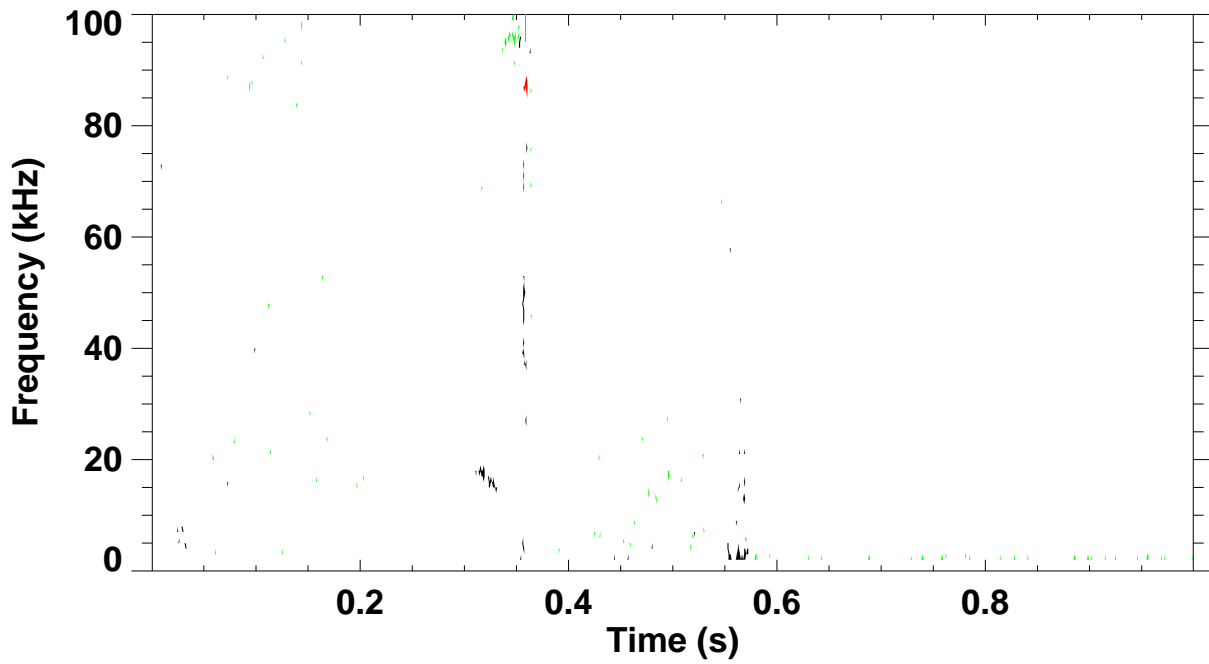
Shot 127451 \omega B(\omega) spectrum for toroidal mode number: 1 2 3 4 5
