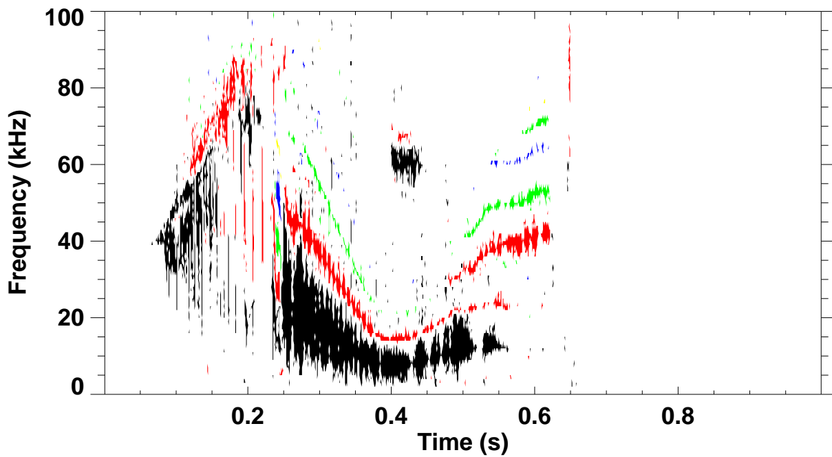
Shot 127956 \omega_B(\omega) spectrum for toroidal mode number: 1 2 3 4 5
