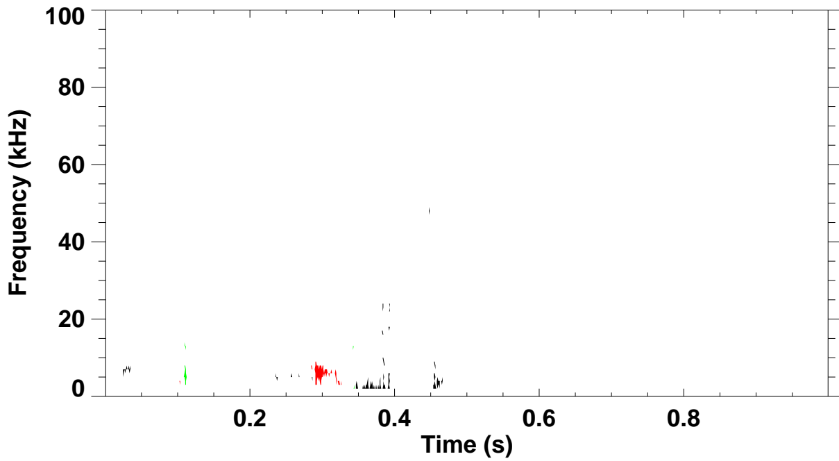
Shot 127959 \omega B(\omega) spectrum for toroidal mode number: 1 2 3 4 5
