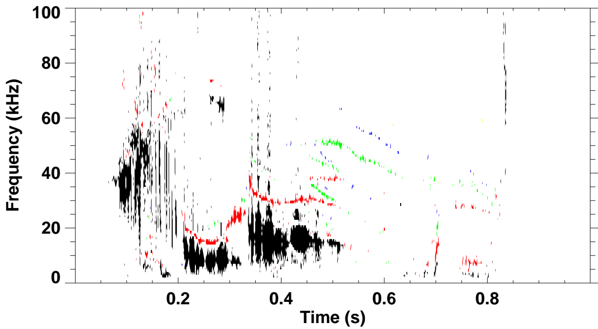
Shot 127975 \omega B(\omega) spectrum for toroidal mode number: 1 2 3 4 5
