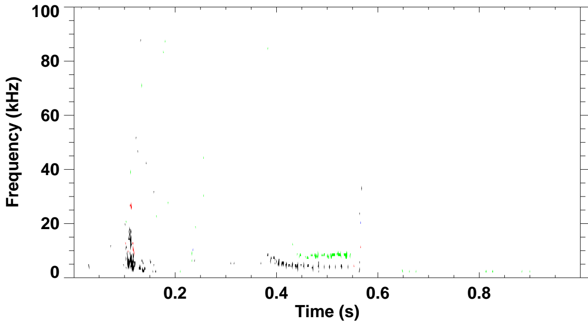
Shot 128139 \omega B(\omega) spectrum for toroidal mode number: 1 2 3 4 5
