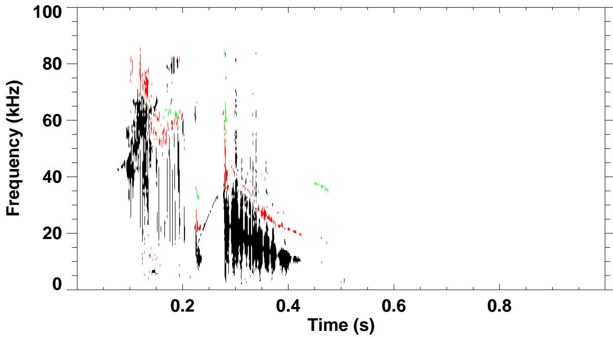
Shot 128641 \omega B(\omega) spectrum for toroidal mode number: 1 2 3 4 5
