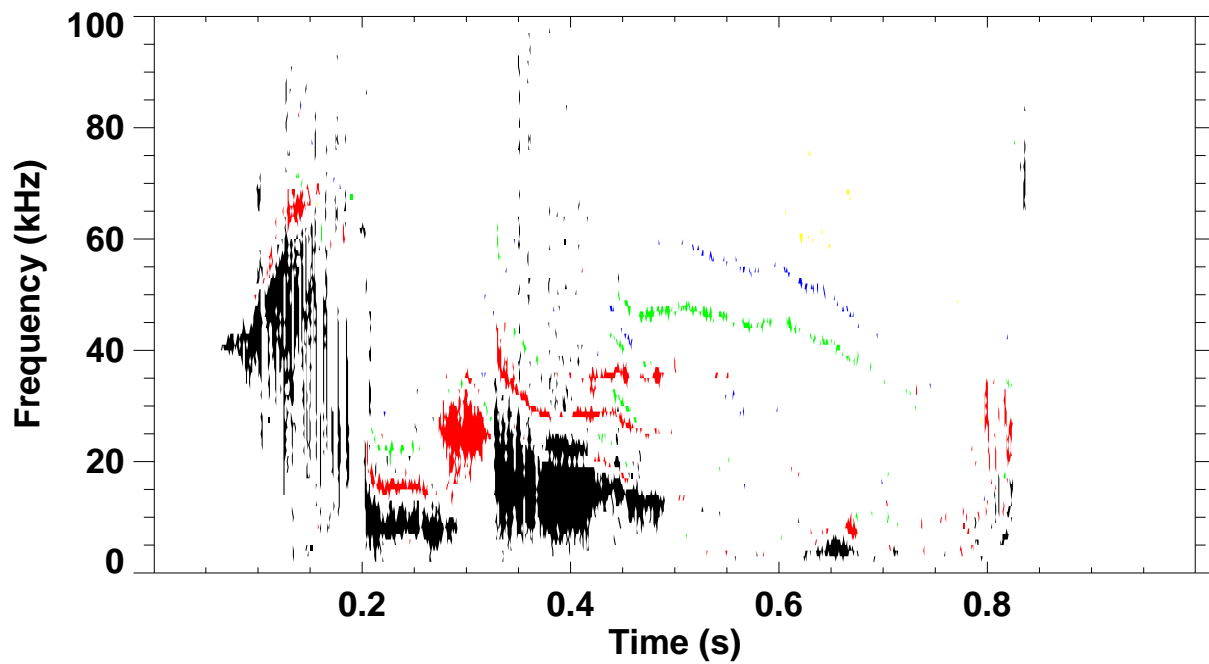
Shot 128677 \omega B(\omega) spectrum for toroidal mode number: 1 2 3 4 5
