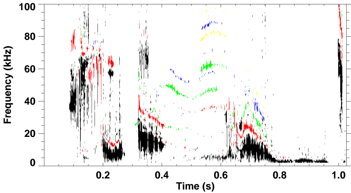
Shot 128692 \omega B(\omega) spectrum for toroidal mode number: 1 2 3 4 5
