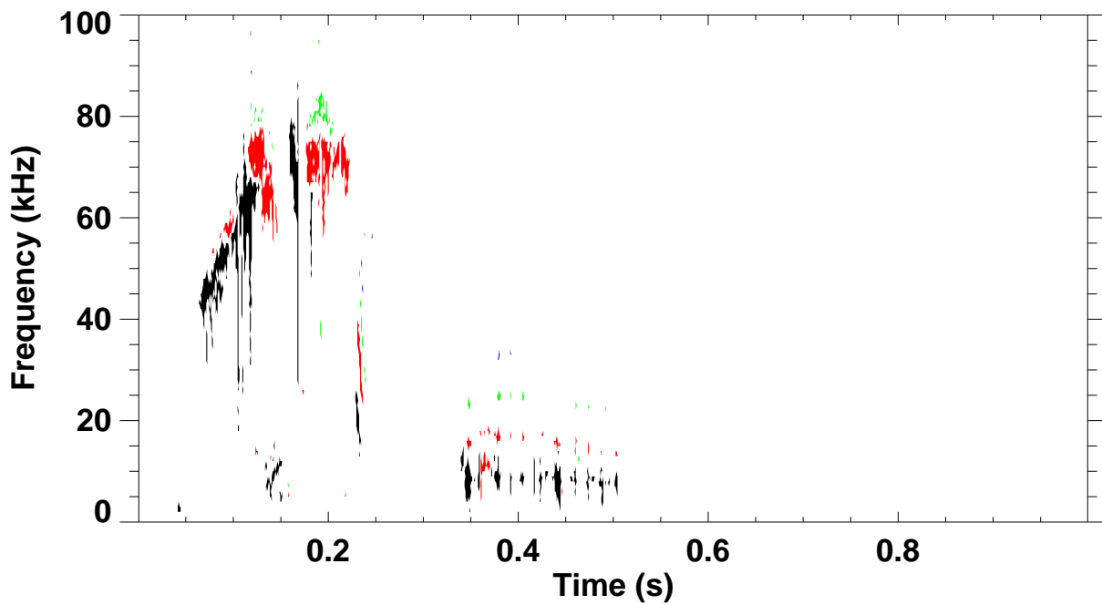
Shot 128779 \omega B(\omega) spectrum for toroidal mode number: 1 2 3 4 5
