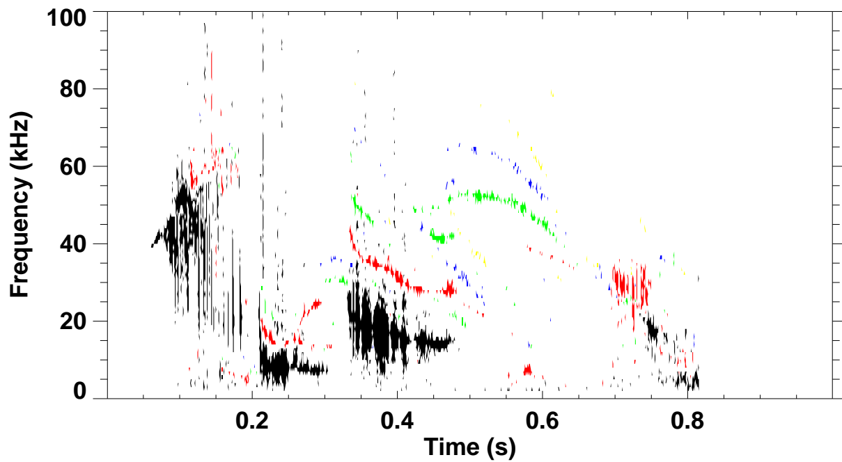
Shot 128802 \omega B(\omega) spectrum for toroidal mode number: 1 2 3 4 5
