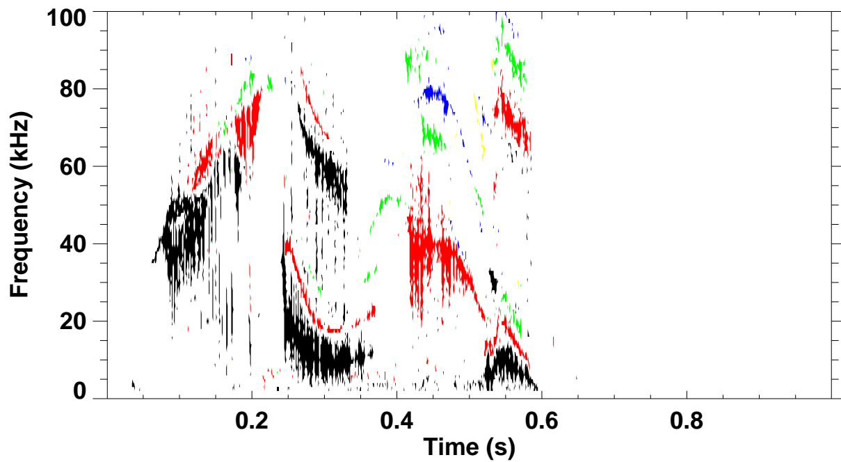
Shot 128826 \omega B(\omega) spectrum for toroidal mode number: 1 2 3 4 5
