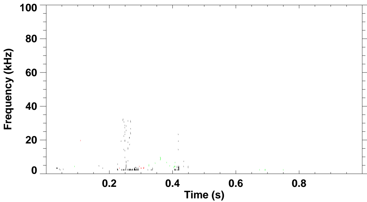
Shot 128959 \omega_B(\omega) spectrum for toroidal mode number: 1 2 3 4 5
