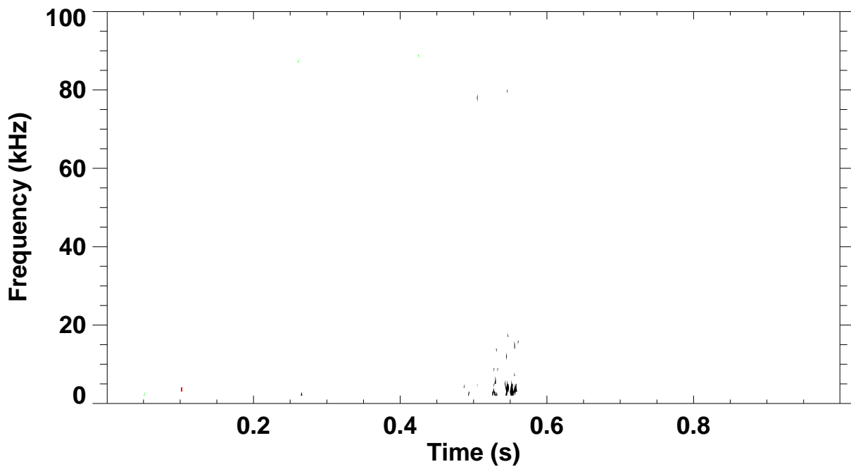
Shot 129000 \omega B(\omega) spectrum for toroidal mode number: 1 2 3 4 5
