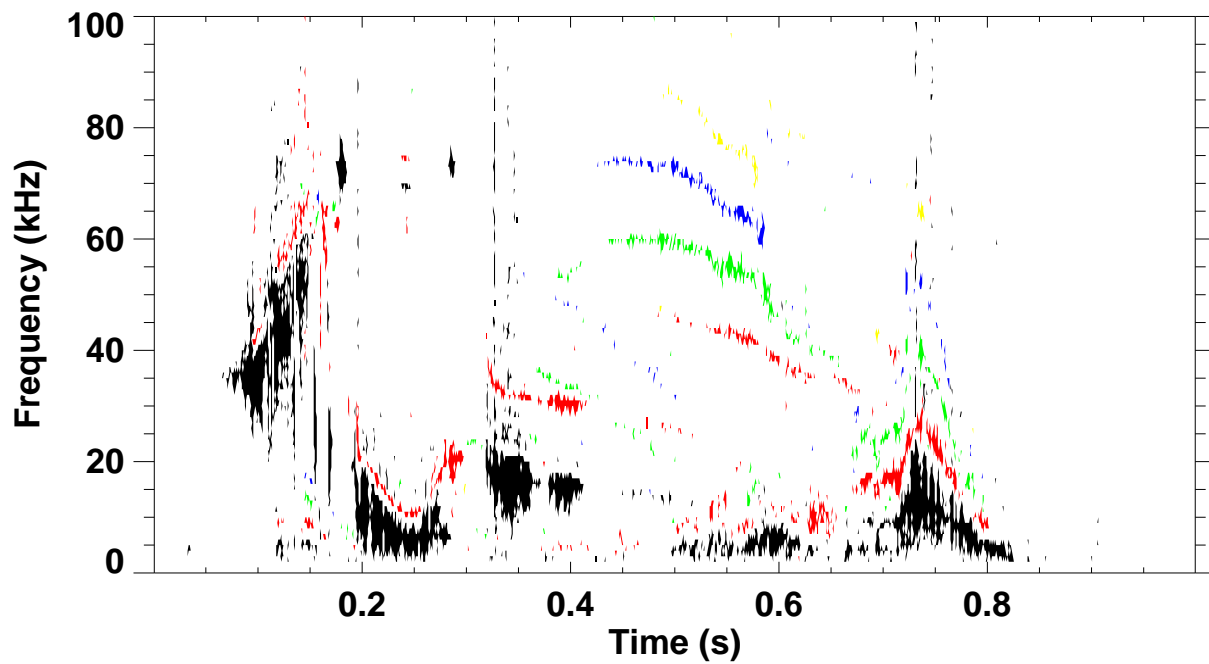
Shot 129237 \omega B(\omega) spectrum for toroidal mode number: 1 2 3 4 5
