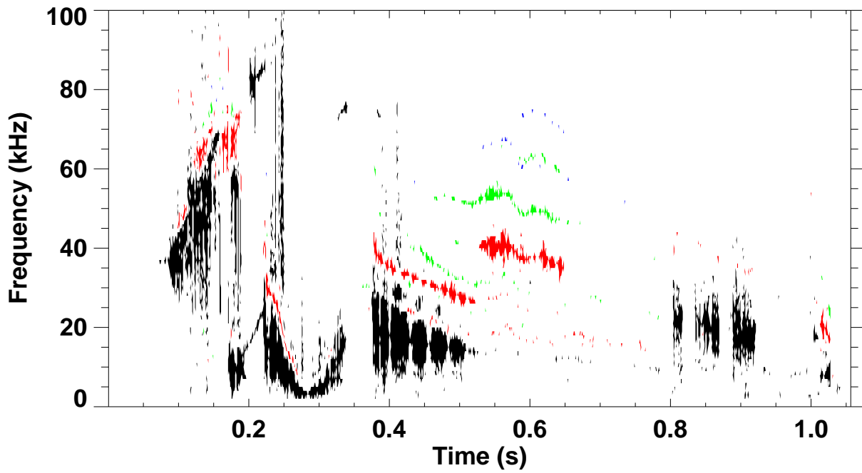
Shot 129317 \omega_B(\omega) spectrum for toroidal mode number: 1 2 3 4 5
