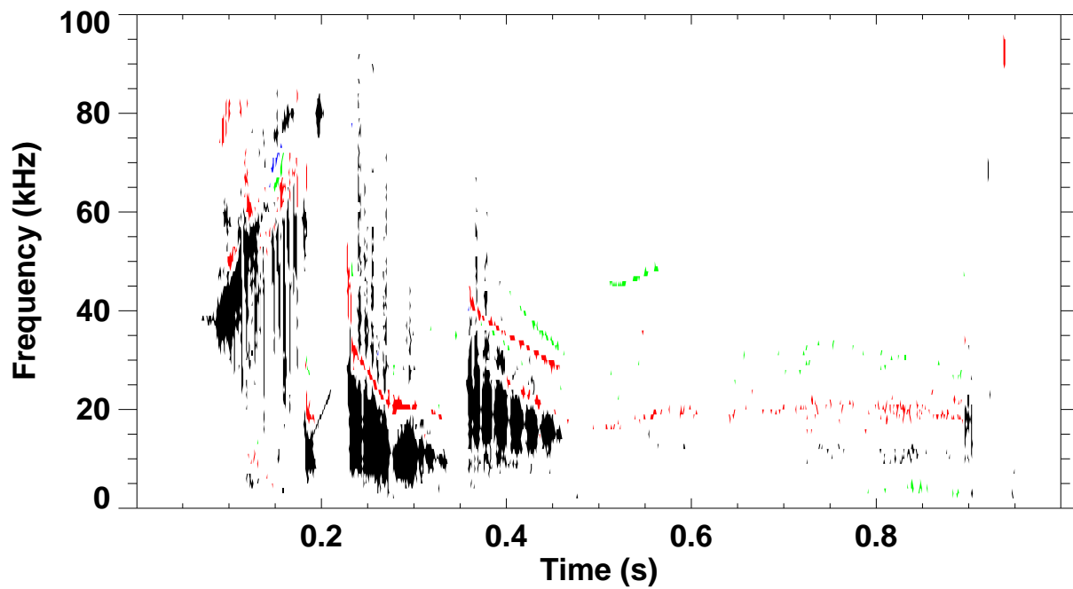
Shot 129860 \omega B(\omega) spectrum for toroidal mode number: 1 2 3 4 5
