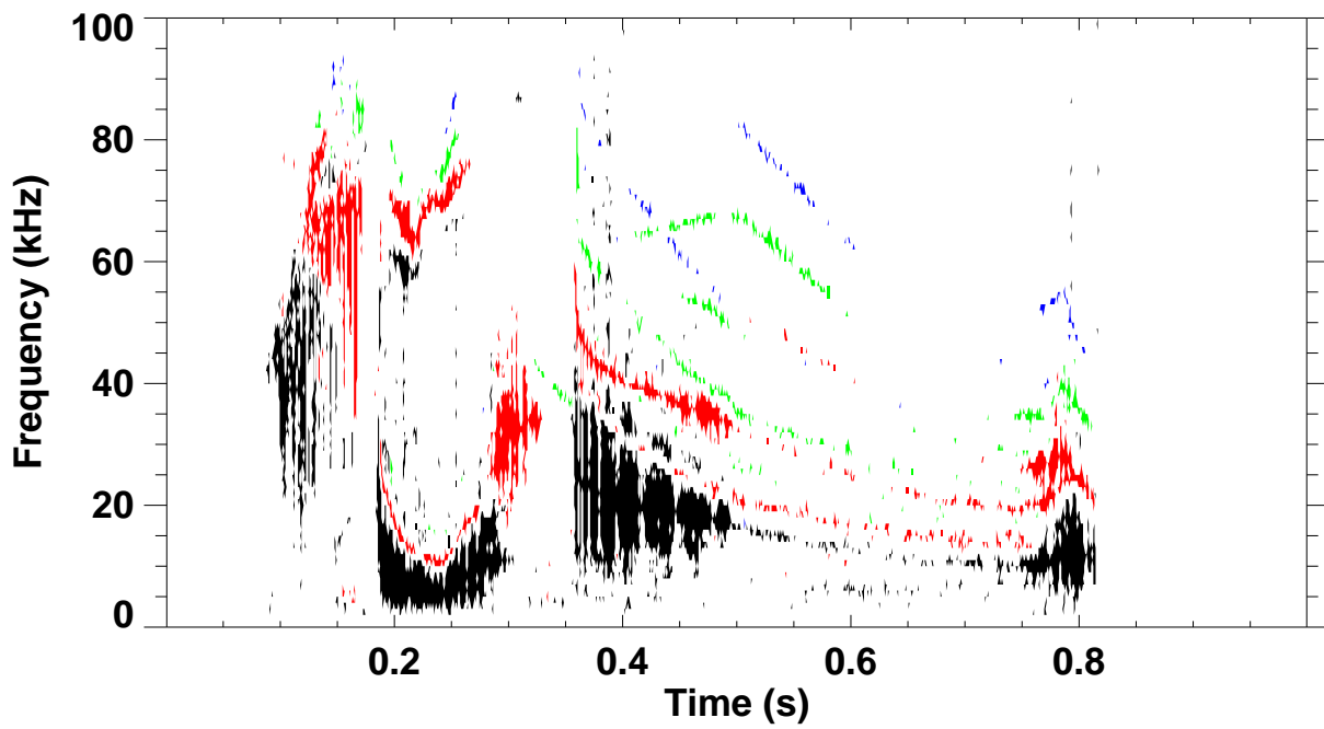
Shot 129904 \omega B(\omega) spectrum for toroidal mode number: 1 2 3 4 5
