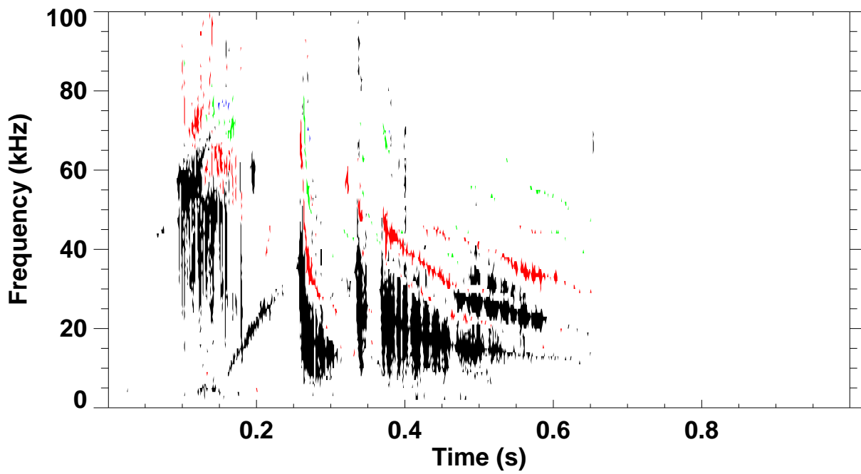
Shot 129932 \omega_B(\omega) spectrum for toroidal mode number: 1 2 3 4 5
