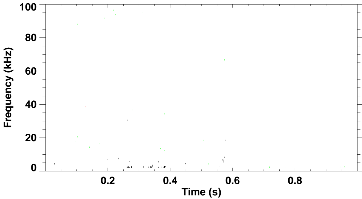
Shot 130116 \omega B(\omega) spectrum for toroidal mode number: 1 2 3 4 5
