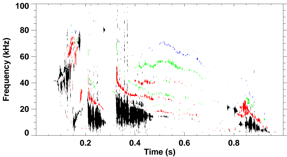
Shot 130190 \omega B(\omega) spectrum for toroidal mode number: 1 2 3 4 5
