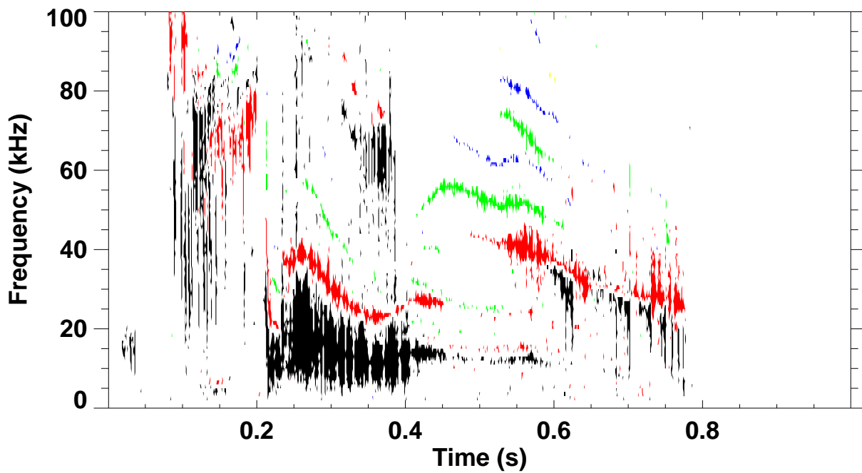
Shot 130226 \omega B(\omega) spectrum for toroidal mode number: 1 2 3 4 5
