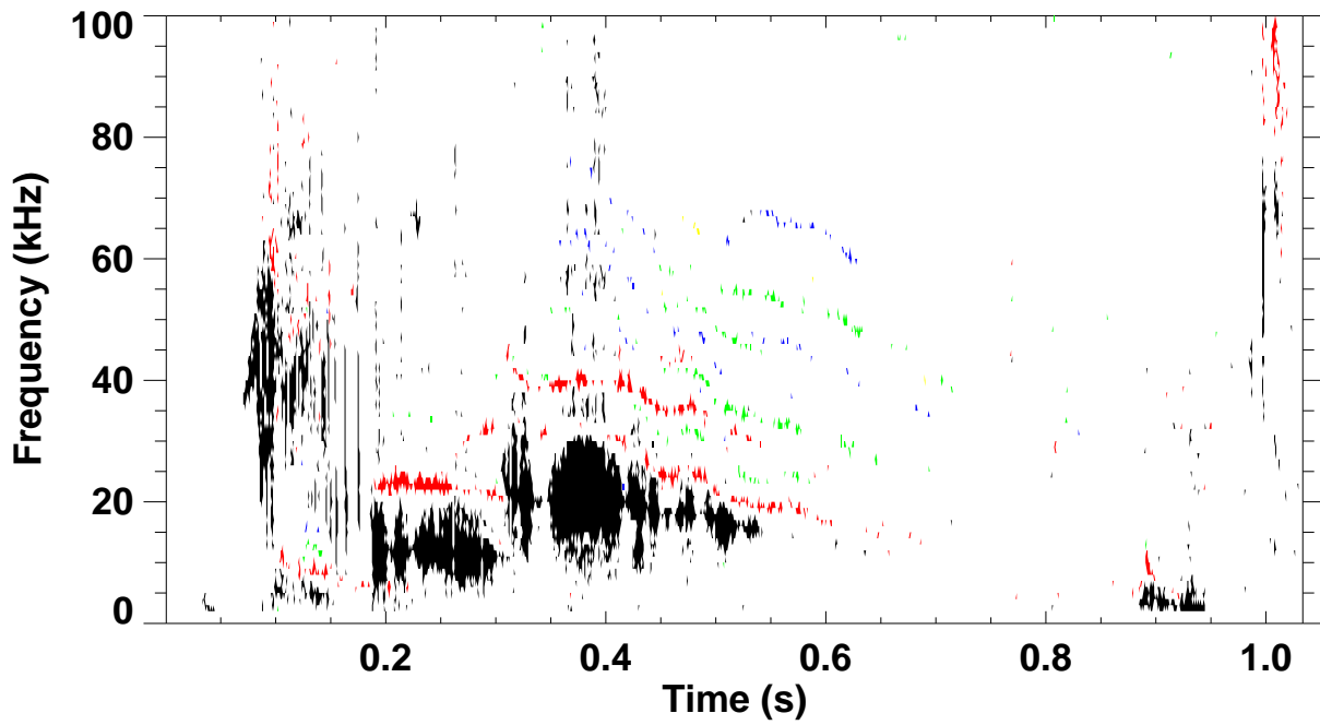
Shot 130241 \omega B(\omega) spectrum for toroidal mode number: 1 2 3 4 5
