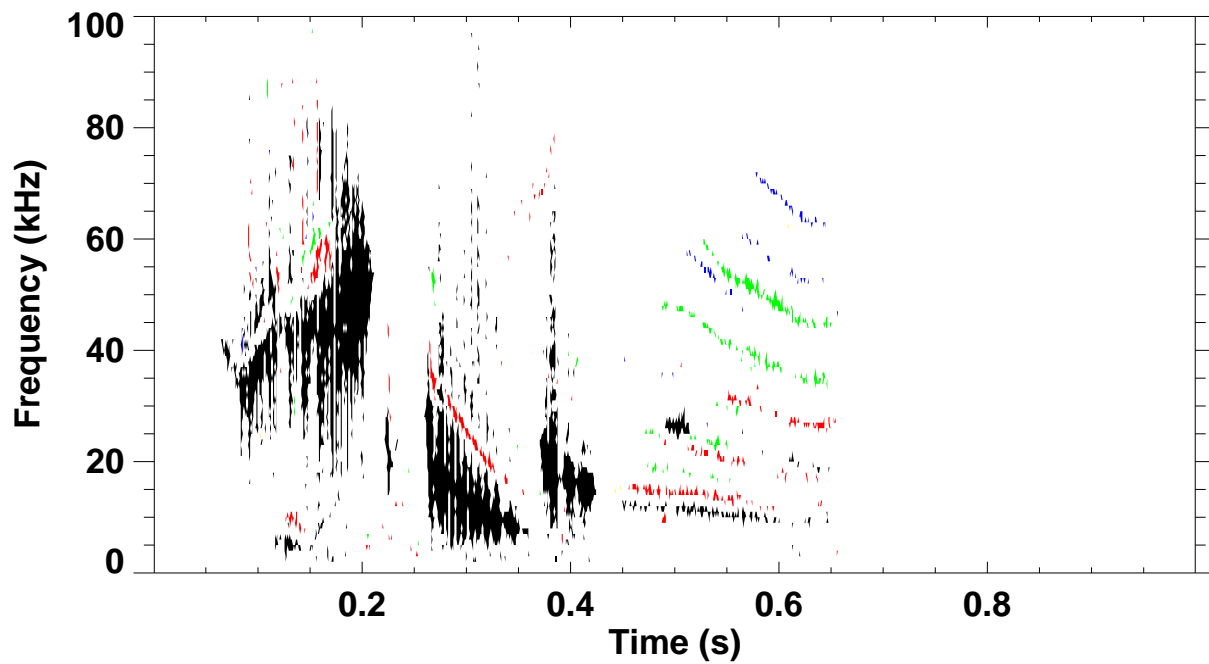
Shot 130350 \omega B(\omega) spectrum for toroidal mode number: 1 2 3 4 5
