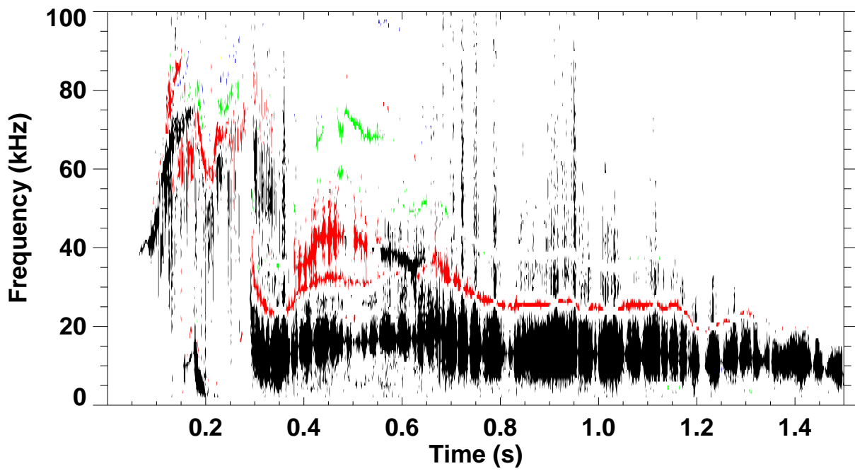
Shot 130400 \omega B(\omega) spectrum for toroidal mode number:
