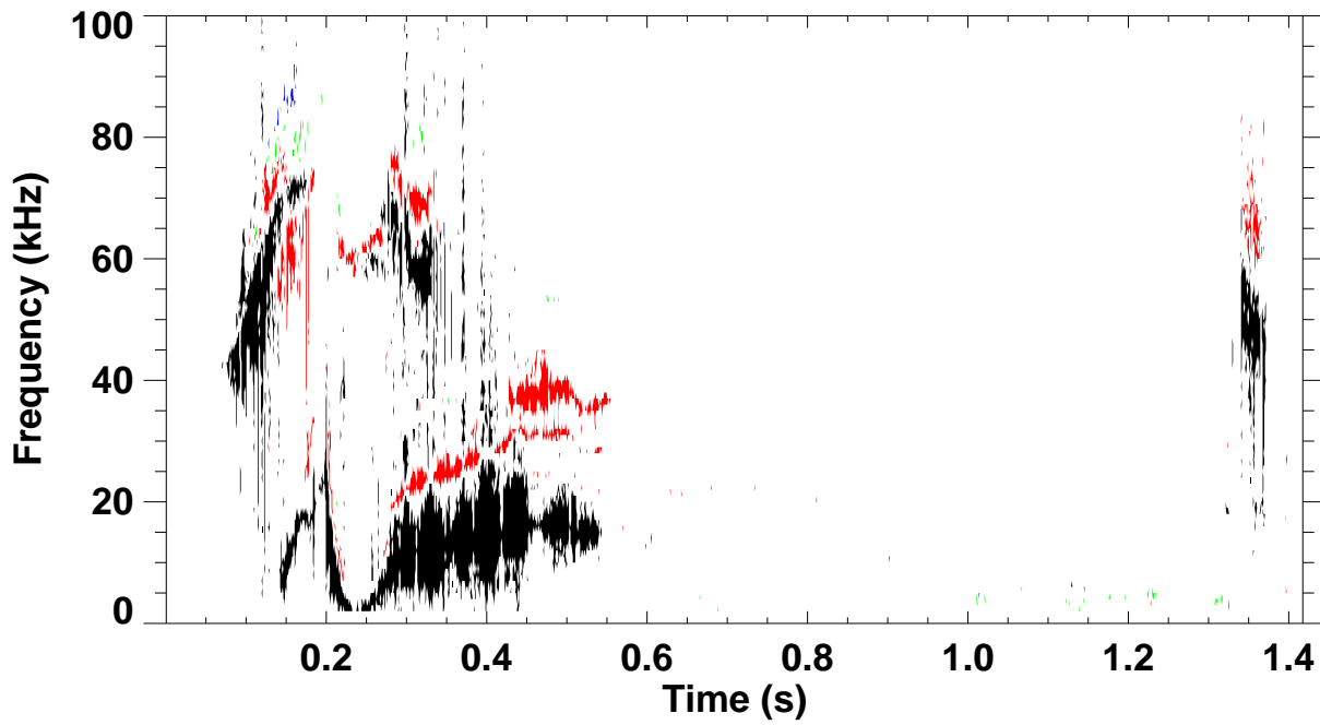
Shot 130406 \omega B(\omega) spectrum for toroidal mode number: 1 2 3 4 5
