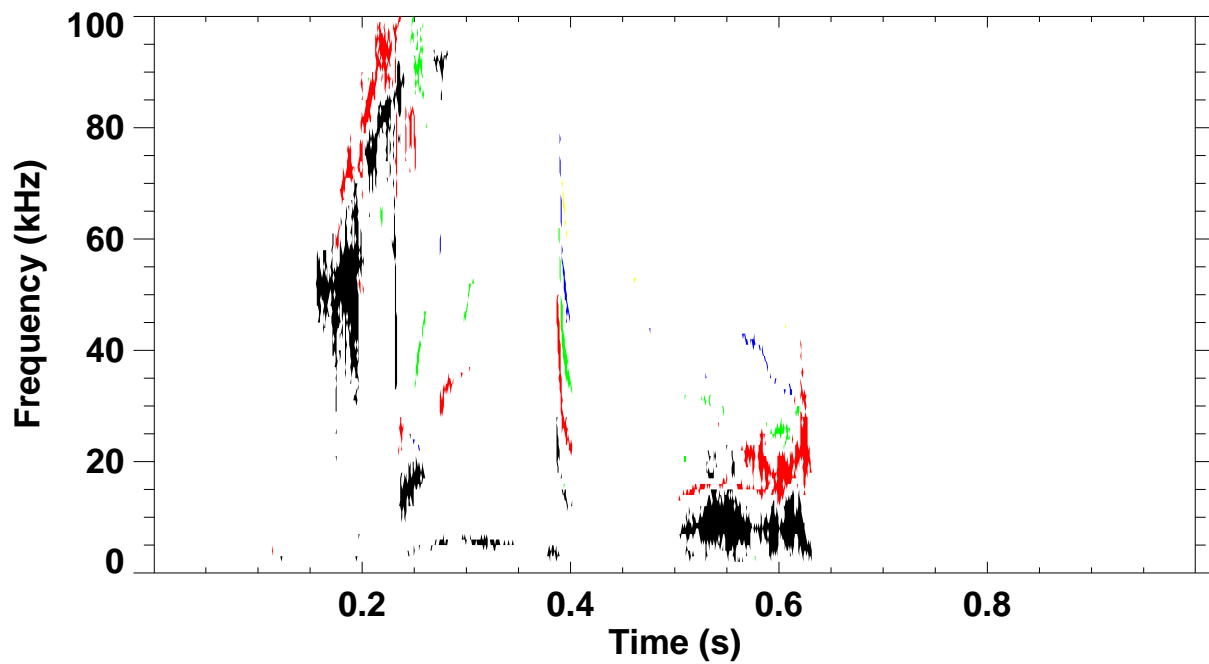
Shot 130608 \omega B(\omega) spectrum for toroidal mode number: 1 2 3 4 5
