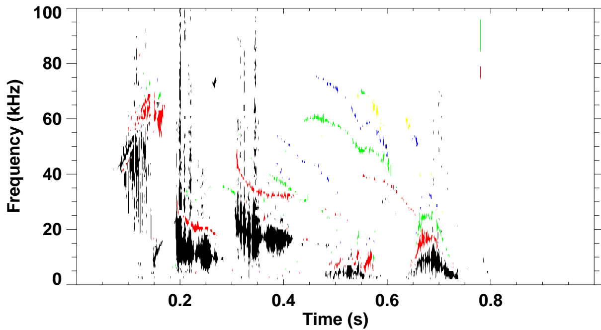
Shot 130719 \omega_B(\omega) spectrum for toroidal mode number: 1 2 3 4 5
