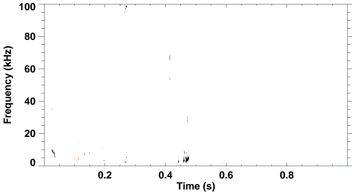
Shot 138339 \omega_B(\omega) spectrum for toroidal mode number: 1 2 3 4 5
